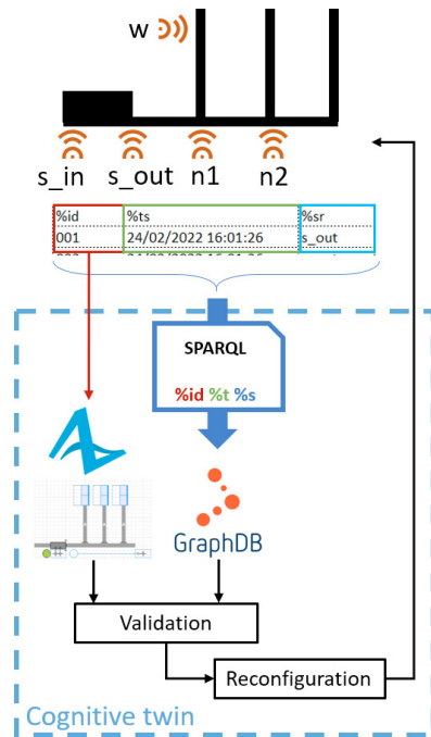
Figure 3 – Architecture of the CT
