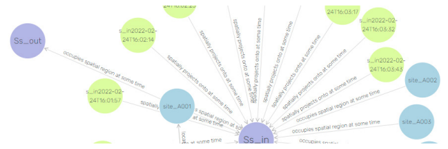
Figure 4 - Snapshot of the KG containing data related to workpiece ID001 in space s\_in
