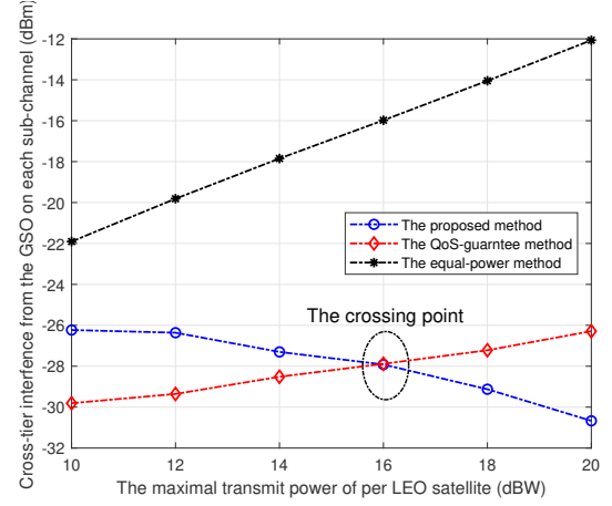
Figure 7. Cross-tier interference from GSO satellite to user terminals in each subchannel.
