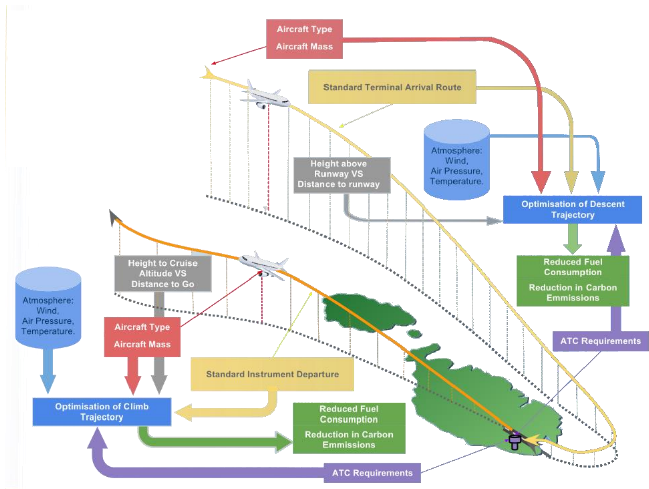
Fig. 1. CFO Process System Overview
