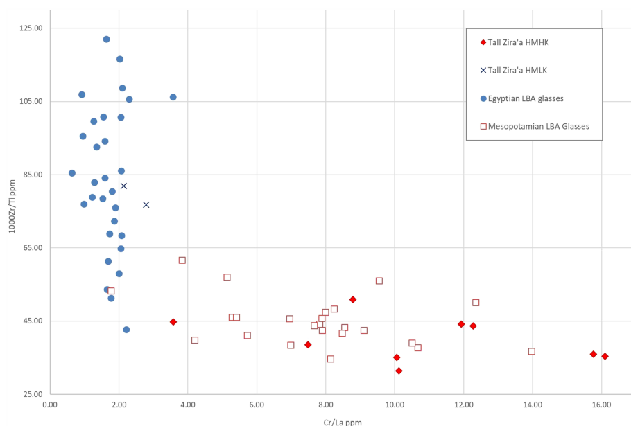
Figure 2 Covariant plot of 1000 Zr/Ti with Cr/La of the Tall Zirā'a high magnesia/high potash (HMK) and high magnesia/low potash (HMLK) groups compared with Egyptian and Mesopotamian glasses of known origin. Source: Shortland et al. (2007). [Colour figure can be viewed at wileyonlinelibrary.com ]
