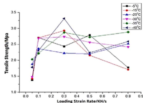
Fig. 8 Relationship between tensile strength and loading rate. 23
