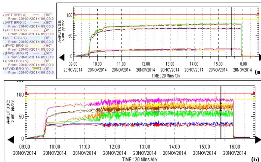
Figure 14. Recorded vibration trends at forward and afterward bearings of: (a) First process stage; (b) Intermediate process stage.
