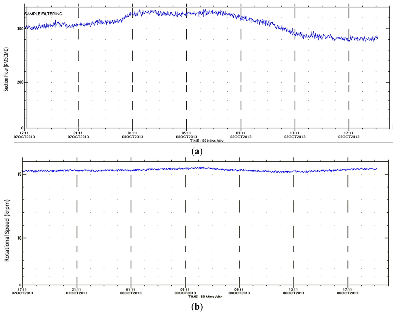
Figure 3. Measured performance parameters of the first process stage: (a) suction flow; (b) rotational speed.
