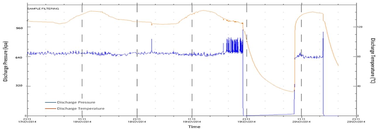
Figure 17. Recorded discharge pressure and temperature.
