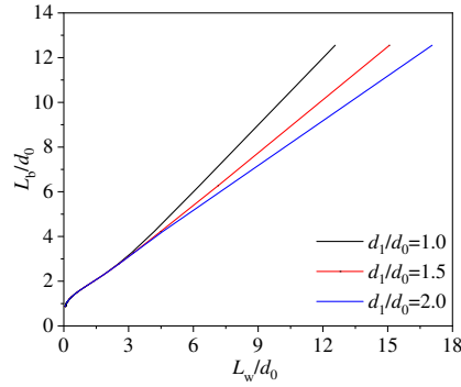
FIG. 11: Implicit function F(L_w, L_b) that forms a one-to-one mapping of L_b and L_w for stepped seabed situations. A larger ratio of d_1/d_0 corresponds to a smaller L'_w , and subsequently a smaller L_b .
