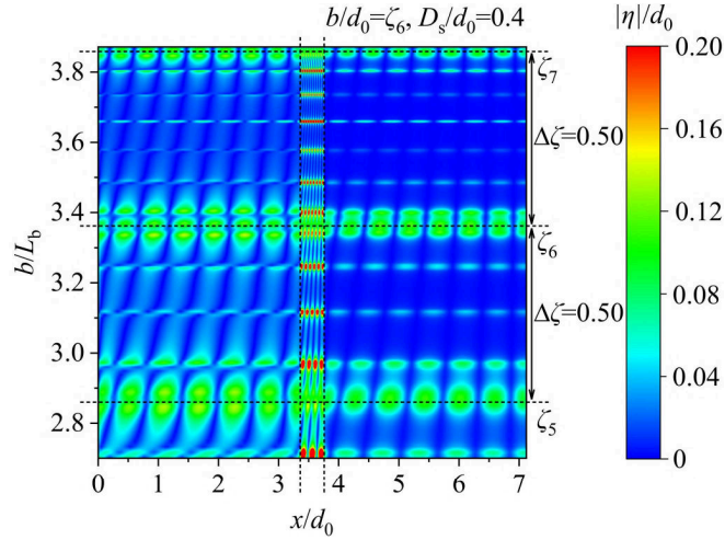
FIG. 19: Oscillation amplitudes of elements along Patch-1 and Patch-2 and of free surface in different wave conditions, with b/d_0 = \xi_6 , D_s/D_0 = 0.4 , and wave conditions represented by b/L_b . In each resonance condition, the oscillation of Patch-1 is evidently weakened compared with the behavior of an isolated Patch-1 in the same wave conditions.
