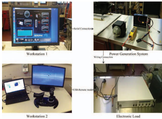
Fig. 10. Hardware-in-the-loop setup.
