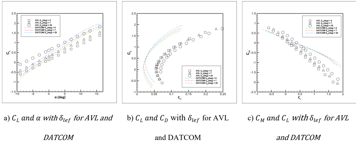
Figure 10 Aerodynamic coefficient analysis comparing the effects of flap deflection on lift C_L , drag C_D and pitching moment C_m coefficients, using AVL and DATCOM simulations. The graphs show the influence of various flap deflections on these coefficients.
