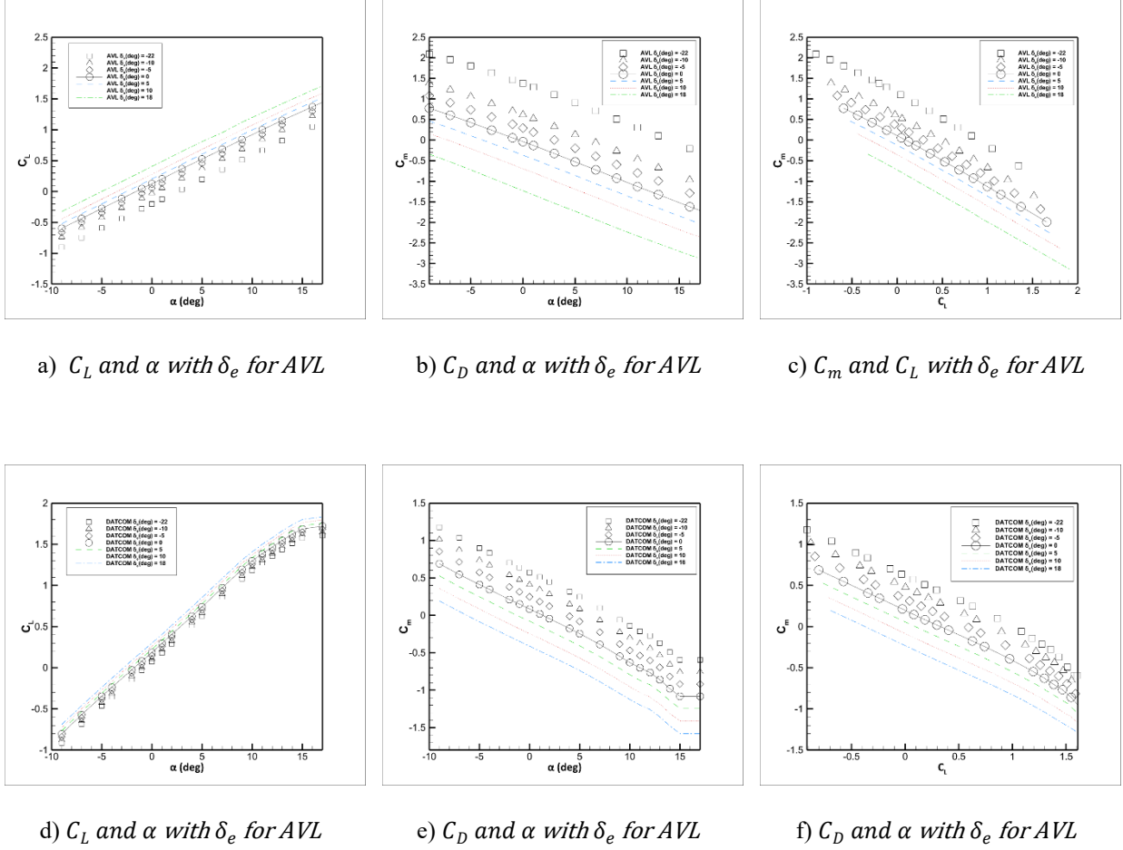
Figure 12 Comparative analysis of the effects of elevator deflections on aerodynamic coefficients using AVL and DATCOM simulations. The graphs demonstrate the relationship between lift ( C_L ), drag ( C_D ), and pitching moment ( C_m ) coefficients with varying angles of attack ( \alpha ) and elevator deflections ( \delta_e ), reflecting the critical role of elevator position in controlling aircraft pitch and lift, with minimal influence on drag.
