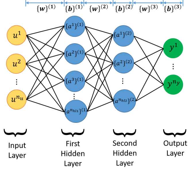
Figure 6 Simple neural network structure.
