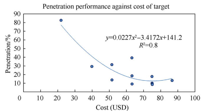
Fig. 9. Penetration mitigation performance against cost of multi-layered targets when subject to high velocity impact loading from a solid steel projectile.
