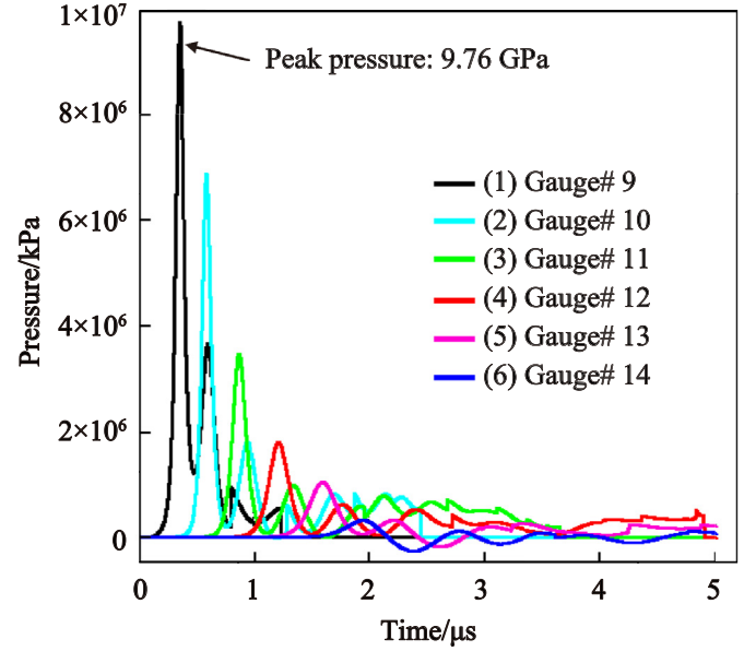
Fig. 3. Peak pressure at different locations on the target against time when steel projectile impacts polycarbonate plate.
