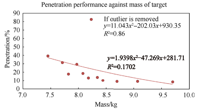
Fig. 8. Penetration mitigation performance against mass of multi-layered targets when subject to high velocity impact loading from a solid steel projectile.
