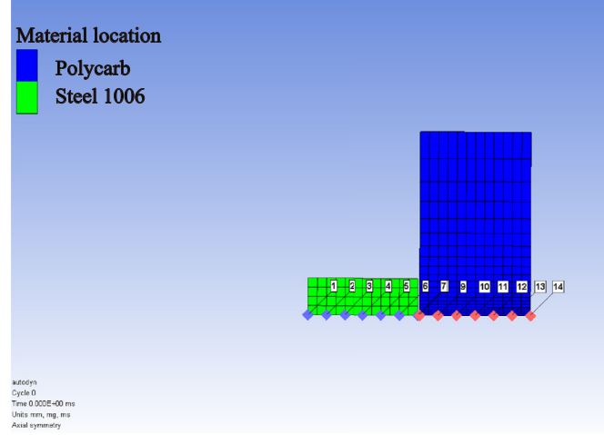
Fig. 2. Code validation set up using a sample model for high velocity impact between steel projectile (Green) and polycarbonate target (Blue).
