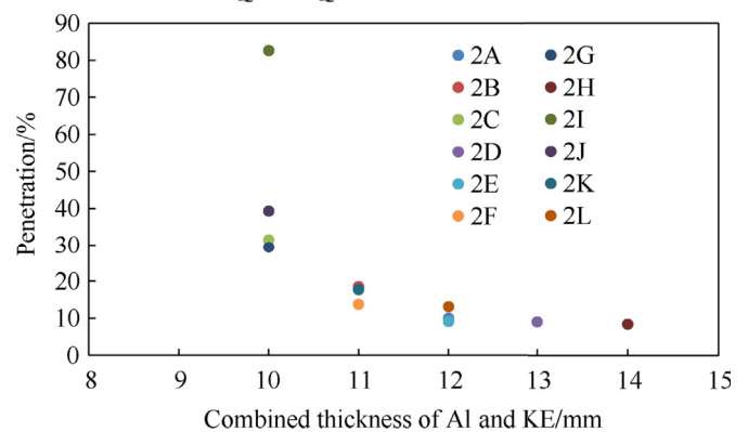
Fig. 7. Penetration mitigation against the combined thickness of Al/KE layers when a multi-layered target is subject to high velocity impact from a steel projectile.
