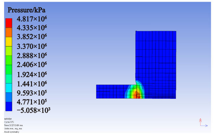
Fig. 4. Pressure gradient at the interface between steel projectile and polycarbonate plate at 3.3 \times 10^{-4} ms during a high velocity impact event.
