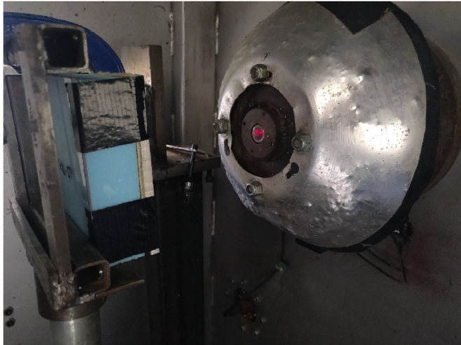
Fig. 5. Multi-layer target setup in ELVIS before being impacted by 5 mm steel projectile at 400 m/s. The target face is Aluminium, followed by Kevlar-Epoxy, Polyurethane foam, and polycarbonate.
