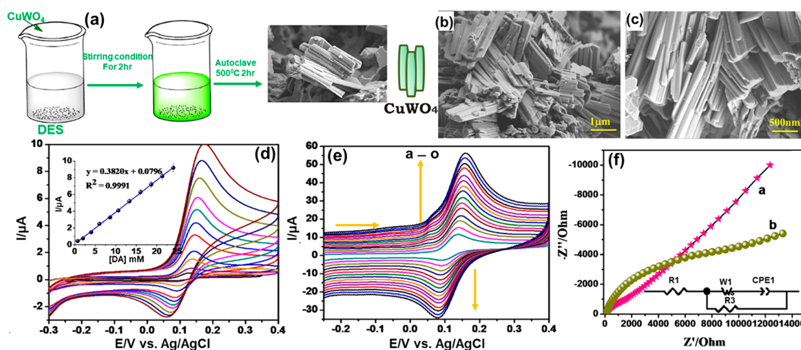
Figure 7. Graphical representation of the \text{CuWO}_4 nanorods' sensor (a); fast electron SEM images of \text{CuWO}_4 nanorods (b, c); CV images at a sweep rate of 50 mV/s for different concentrations of DA and 0.1 mM DA at a sweep rate of 10–300 mV/s (d, e); electrochemical impedance spectra (f). Reprinted with permission from ref 60. Copyright 2022 Elsevier.
