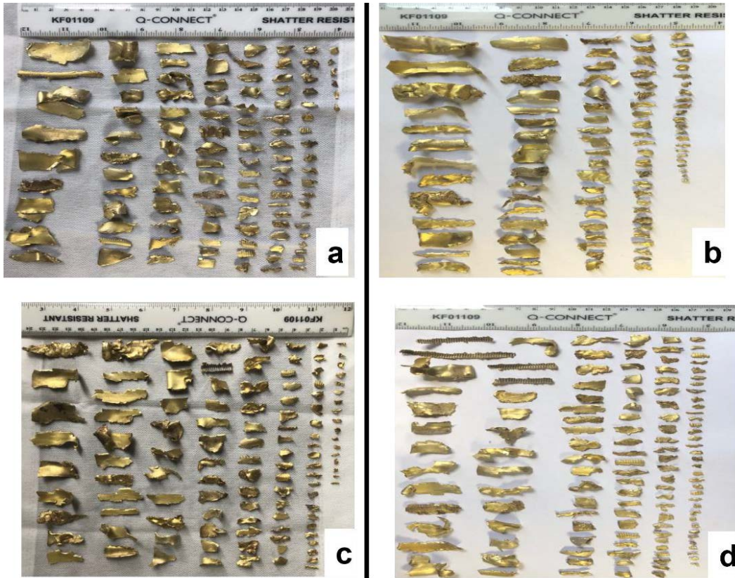
Figure 4. Brass pipe bomb fragments; a) #1 & c) #2 end initiation; b) #3 & d) #4 mid initiation
