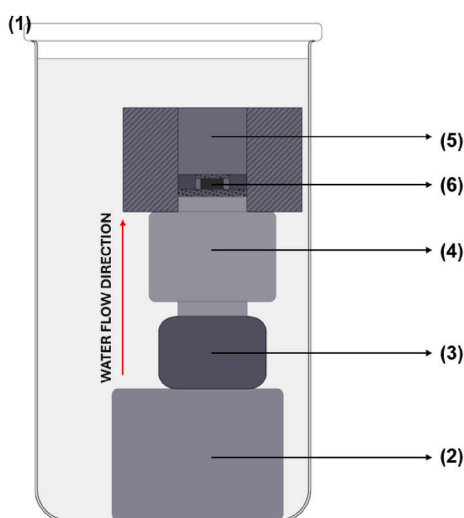
Fig. 1. Experimental set up to examine the dissolution rate of TNT in water showing a 600 mL glass beaker filled (1) with 500 mL distilled water or seawater. Inside the beaker the aquarium pump (2) connected via a Delrin connector (3) to a flowmeter (4) with a PVC holder on top (5). TNT fragment (6) was placed in the PVC holder (5).
