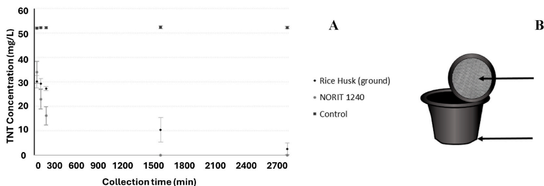
Fig. 4. – A – TNT concentration in mg/l after being in contact with ground rice husk and Norit 1240, placed in a contained environment, collection time (min). B – Enclosed environment with mesh at the top and bottom of the pod. All results are presented with standard deviation.
