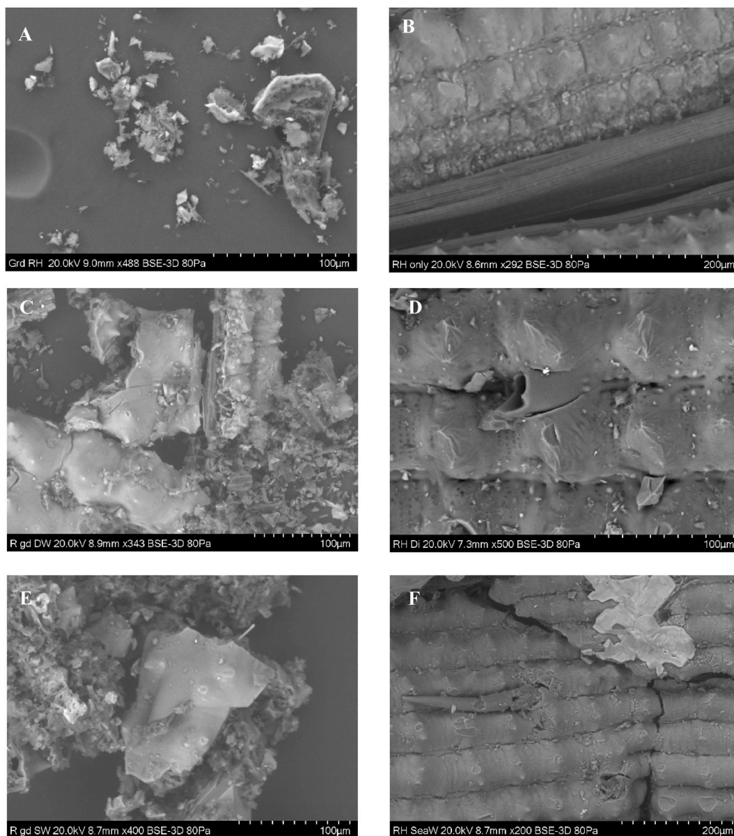
Fig. 3. – SEM images for A- Ground rice husk; B- rice husk; C – Ground rice husk in Distilled water; D – Rice husk in distilled water; E – Ground rice husk in seawater; F- Rice husk in seawater. Fig. 3D has been further magnified to render the surface area and the structure more visible.
