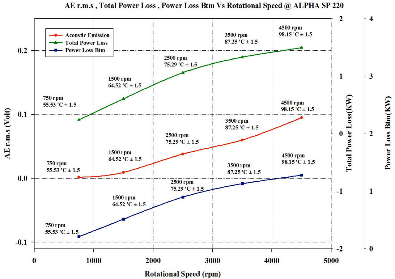
Figure 9 AE r.m.s, rotational speed, dynamic viscosity (SP220), bottom power losses and total loss for load condition 10KN
