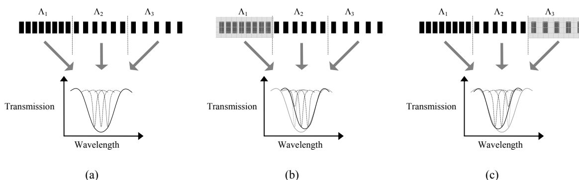
Figure 1. Simplified representation of a chirped LPG; (a) shows the composite band formed from the three closely matched but different period LPGs, (b) the effect of covering the section of the LPG with a period of \Lambda_1 , (c) the effect of covering the section of the LPG with a period of \Lambda_3 .
