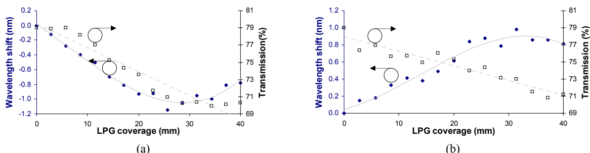
Figure 5. Wavelength shift (♦) of band 6 and minimum transmission value (□) against LPG coverage with Cargille index oil (1.56) for LPG arranged with decreasing period (a) and increasing period (b). Grey lines are shown only as a visual aid.
