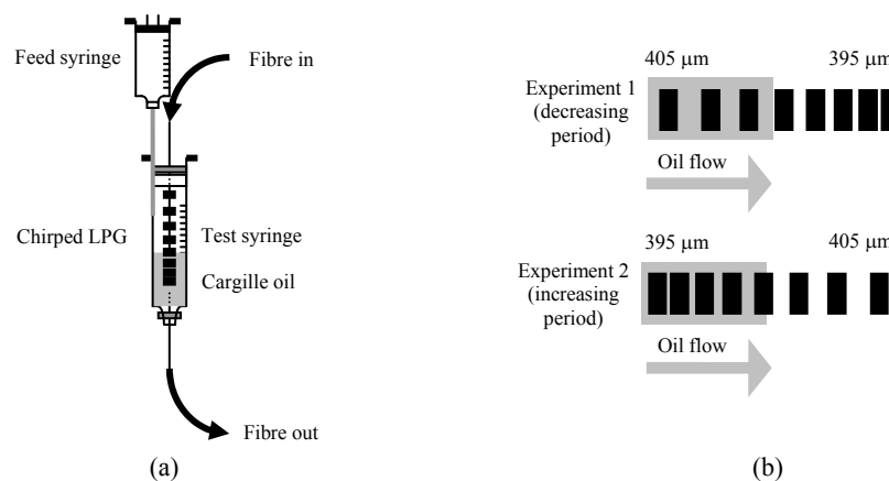
Figure 3. Experimental setup for chirped long period grating flow sensor (a) orientation of the chirped LPG for the flow sensing experiments (b).
