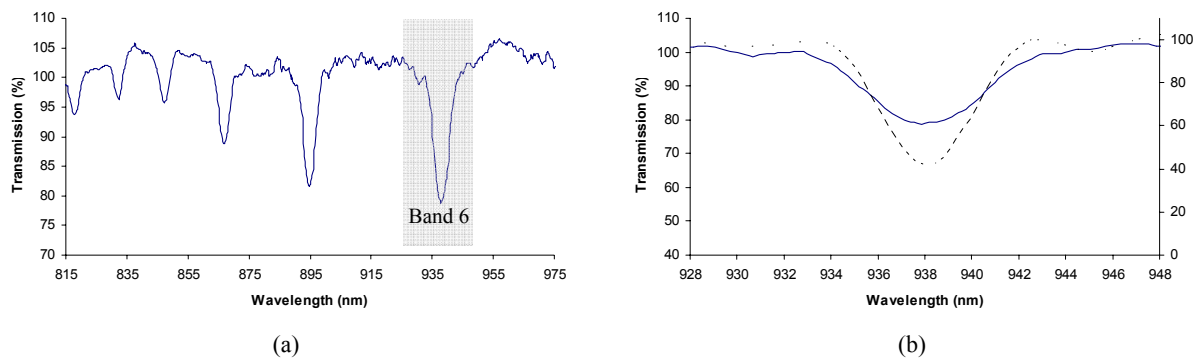
Figure 2. Transmission spectrum of a chirped LPG of length 40mm and linearly chirped period 395 \mu m - 405 \mu m, fabricated in Fibercore SM750. Band 6 is highlighted and shown compared with a band in the same spectral location (b) of an LPG of uniform period 400 \mu m (dashed).
