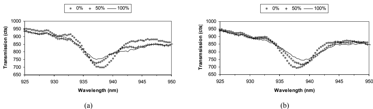
Figure 4. Change in shape of band 6 for gradual immersion in 1.56 Cargille index oil. Experiment 1 (a) and experiment 2 (b). 0% is no coverage, 50% half and 100% total coverage.
