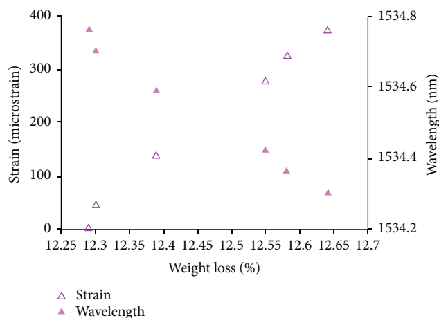
FIGURE 5: A plot of strain and wavelength against weight loss of gel.
