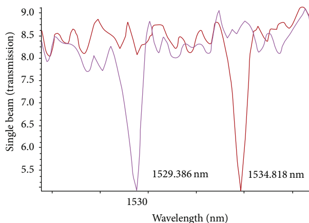
FIGURE 3: Bragg wavelength shift due to drying of gel.
