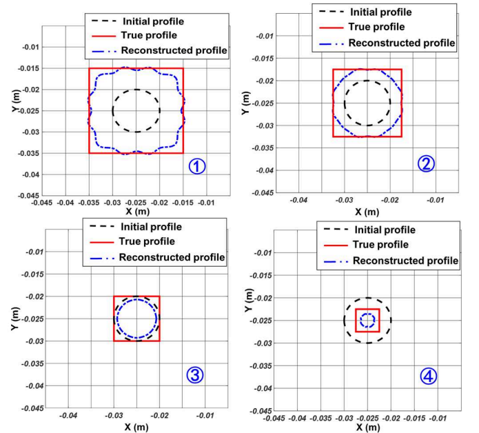
Fig. 13. Reconstruction results of the Al-Cu specimen.
