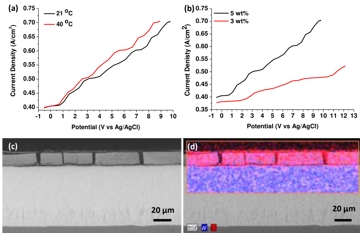
Figure 6: Anodic polarisation curves of W/WC in (a) 5 wt% NaOH electrolyte at temperature of 21 °C and 40 °C and (b) at 21 °C using electrolyte concentration of 5 wt% and 3 wt% NaOH. (c) SEM and (d) corresponding EDS maps of the cross-section showing the formation of WO_3 on W/WC coating under regime II conditions in 5 wt% NaOH solution at room temperature.
