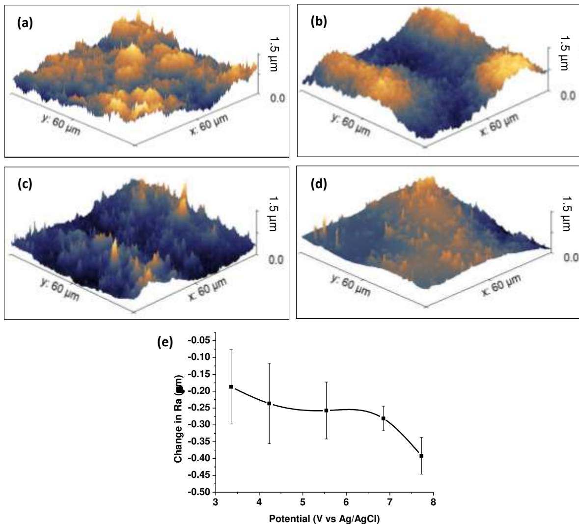
Figure 3: AFM Surface profiles of W/WC coated samples in the (a) as-deposited and electropolished conditions at (b) 3 V vs Ag/AgCl, (c) 5.5 V vs Ag/AgCl and (d) 7.9 V vs Ag/AgCl. (e) Changes in the mean Ra of electropolished W/WC-coated samples vs applied potential vs Ag/AgCl. Zero change in Ra represents the as-deposited condition. The electropolishing conditions for (b)-(e) are 1000 ml of 5 wt% NaOH electrolyte solution at 21 °C for 5 mins. Error bars represent the uncertainties of the measured data.
