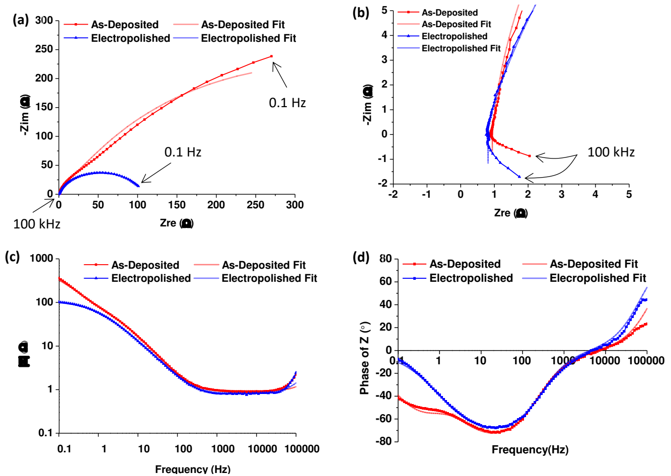
Figure 5: (a) Overall and (b) zoomed-in EIS Nyquist plot, (c) Bode plot and (d) Phase angle vs. log frequency of as-deposited and electropolished W/WC samples obtained at a potential of -0.71 V and -0.61 V vs Ag/AgCl, respectively. Here the samples were electropolished in 5 wt% NaOH with a potential of 7 V vs Ag/AgCl for 2 mins
