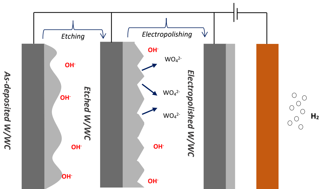
Figure 7: Schematic representation outlining the different electropolishing stages.
