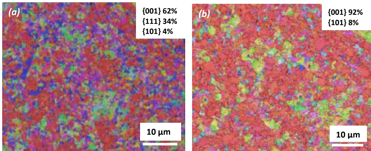
Figure 4: Surface EBSD orientation maps of W/WC coating surface after being (a) mechanically polished using colloidal silica and (b) electropolished in 5 wt% NaOH at 7 V vs Ag/AgCl for 30 s. The mechanically polished W/WC coating exhibits grain distribution of 62% {001}, 34% {111}, and 4% {101}, while the electropolished one exhibits grain distribution of 92% {001} and 8% {101}.
