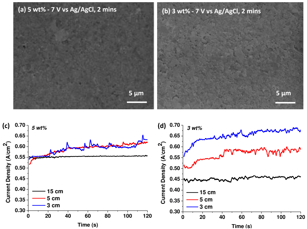
Figure 8: SEM images showing the surface topography of electropolished W/WC coating at a potential of 7 V vs Ag/AgCl for a duration of 2 mins in (a) 5 wt% and (b) 3 wt% NaOH. Variation in time-dependent current density obtained using inter-electrode gap of 3 cm, 5 cm, and 15 cm in (c) 5 wt% and (d) 3 wt% NaOH concentrations at 21 °C with a potential of 7 V vs Ag/AgCl.
