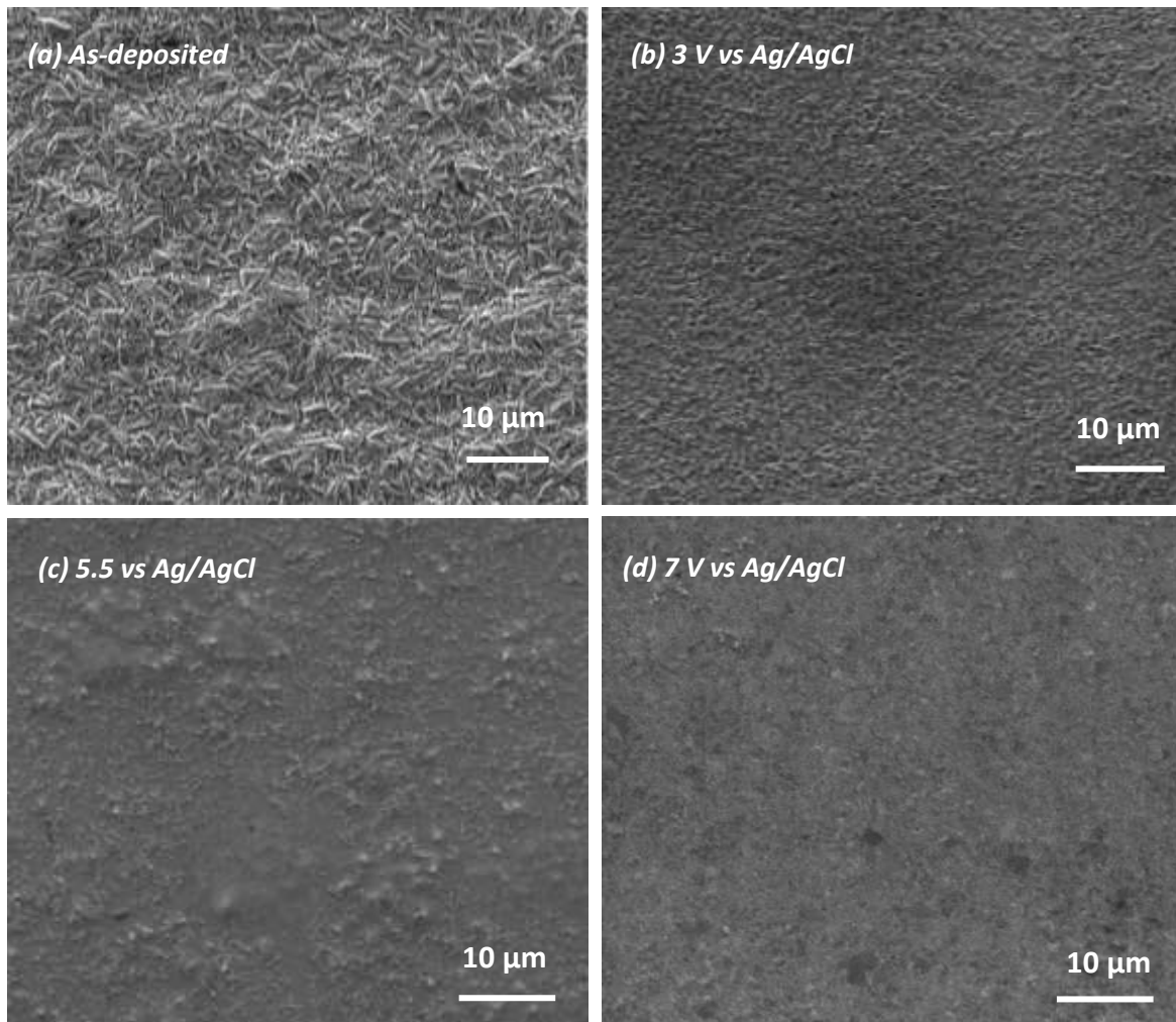
Figure 2: Top view SEM images showing surface morphologies of W/WC coatings (a) as-deposited and after being subjected to electropolishing for 5 mins in 1000 ml of 5 wt% NaOH electrolyte solution at 21 °C at (b) 3 V, (c) 5.5 V, and (d) 7 V vs Ag/AgCl.
