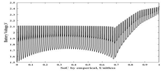
Fig.7 The empirical SoC vs battery voltage curve.
