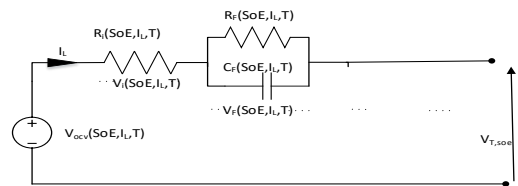
Fig.5 Battery model for SoE estimation
