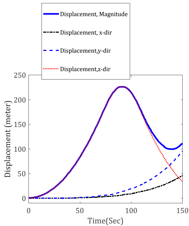
Figure 8. Variation of displacements in the compatibility scenario.
