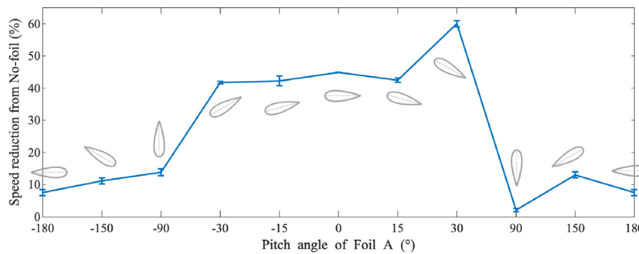
Fig. 10. Comparison of drifting speeds: varied pitch angle of Foil A with vertical Foil B and C. (The y-axis represents the drift speed reduction of the WDP+platform model compared to the No-foil setup, expressed as a percentage, and the x-axis shows the different pitch angles. The grey foil icon illustrates the actual rotational position of Foil A).
