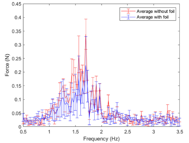
Fig. 18. Average variance in mooring line loads with and without a foil.
