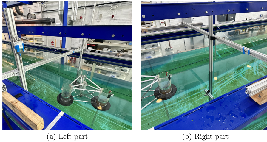
Fig. 14. Photograph of the platform with mooring system placed in the wave tank.
