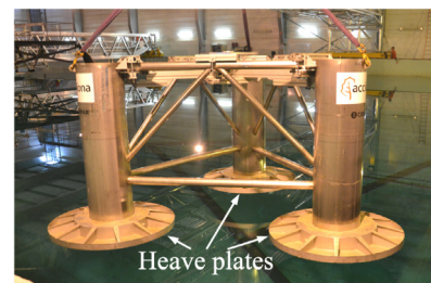
(b) Heave plates under semi-submersible platform [11]
