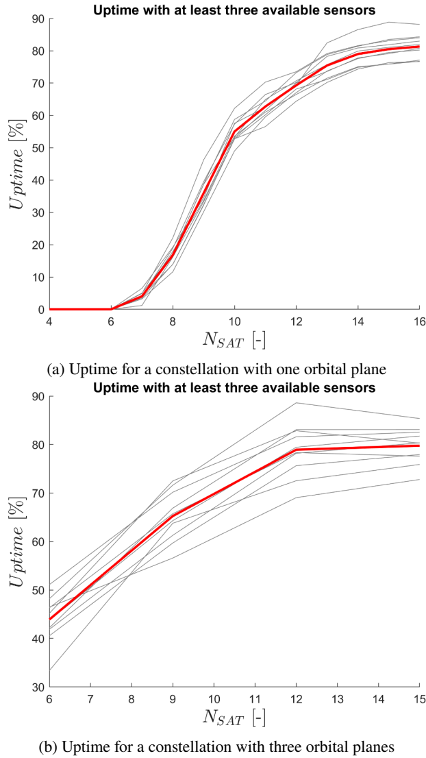
Figure 7: Uptimes against number of spacecraft. Light grey curves indicate a single Monte Carlo run, red curves show the average over the Monte Carlo runs.
