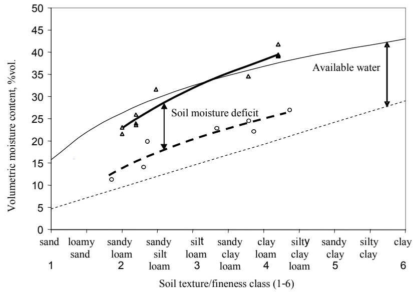
Fig. 3. Volumetric moisture content – soil textural class relationships for EMI surveys at field capacity and after harvest in the field in Fig. 2 (after Waine et al., 2000): \Delta , March 1999; \circ , August 1997; —, UK Field capacity (-0.05 bar); ----, UK Permanent wilting point (-15 bar); - -, Log (March 1999); —, Log, (August 1997)
