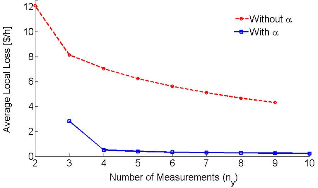
Figure 4: Local average loss for best measurement set with size n_y
