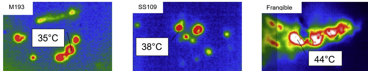
Fig. 15. Under the impact angle of 15°, all projectiles start to fragmentise. In the case of the frangible projectile, a continuous thermal pattern can be recognised. This is the impact angle, where all projectile types show a significant momentum drop.
