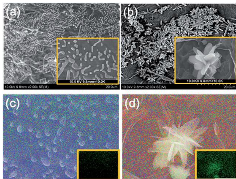
Figure 20. SEM micrograph of (a) graphene/alginate single network and (b) graphene/alginate double network, elemental mapping of (c) graphene/alginate single network, (d) graphene/alginate double network, with insets of mapping of oxygen element (Zhuang et al., 2016). Reproduced from (Zhuang et al., 2016). Published by Royal Society of Chemistry.
