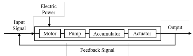
Figure 4. Schematic of a typical EHSA (MOOG)
