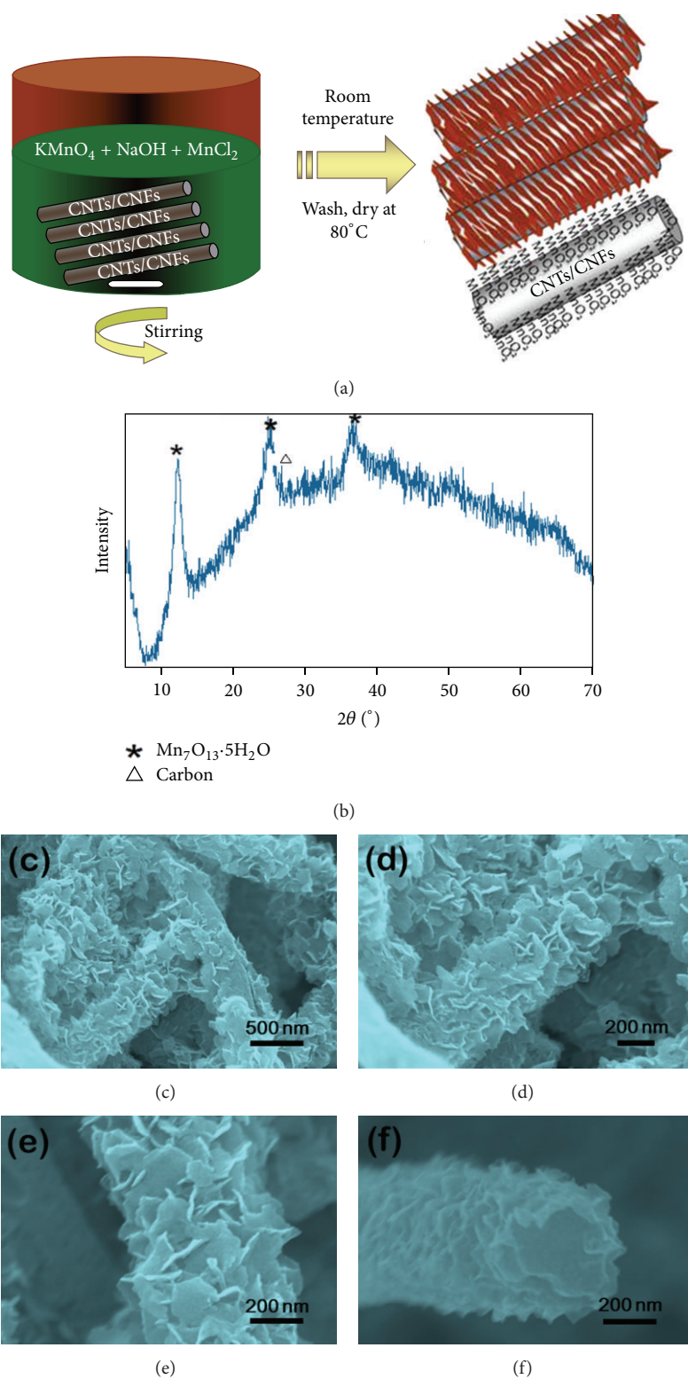
FIGURE 1: (a) Schematic of coating 2D MnO 2 nanosheets onto CNFs surfaces at room temperature. (b) XRD patterns of as prepared CNFs-MnO 2 crystal structures. (c)–(f) SEM images of CNF-MnO 2 mats with different magnifications.
