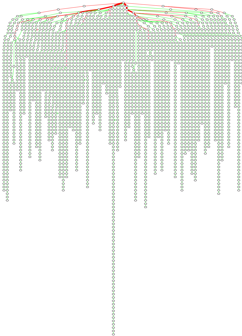
Fig. 4: The directed graph of the board states for one random game per user from the experiment in ordered play
