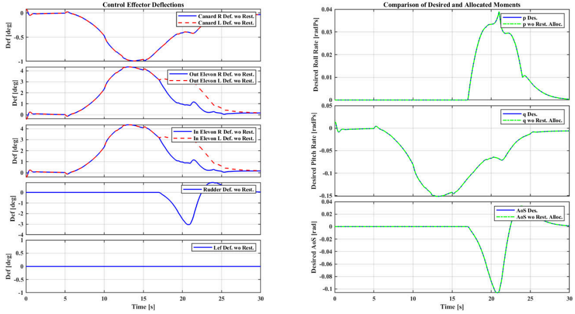
Figure 41: Scenario 2: Closed-Loop Results for Weighted Pseudo-Inverse (Clipped) Approach.
