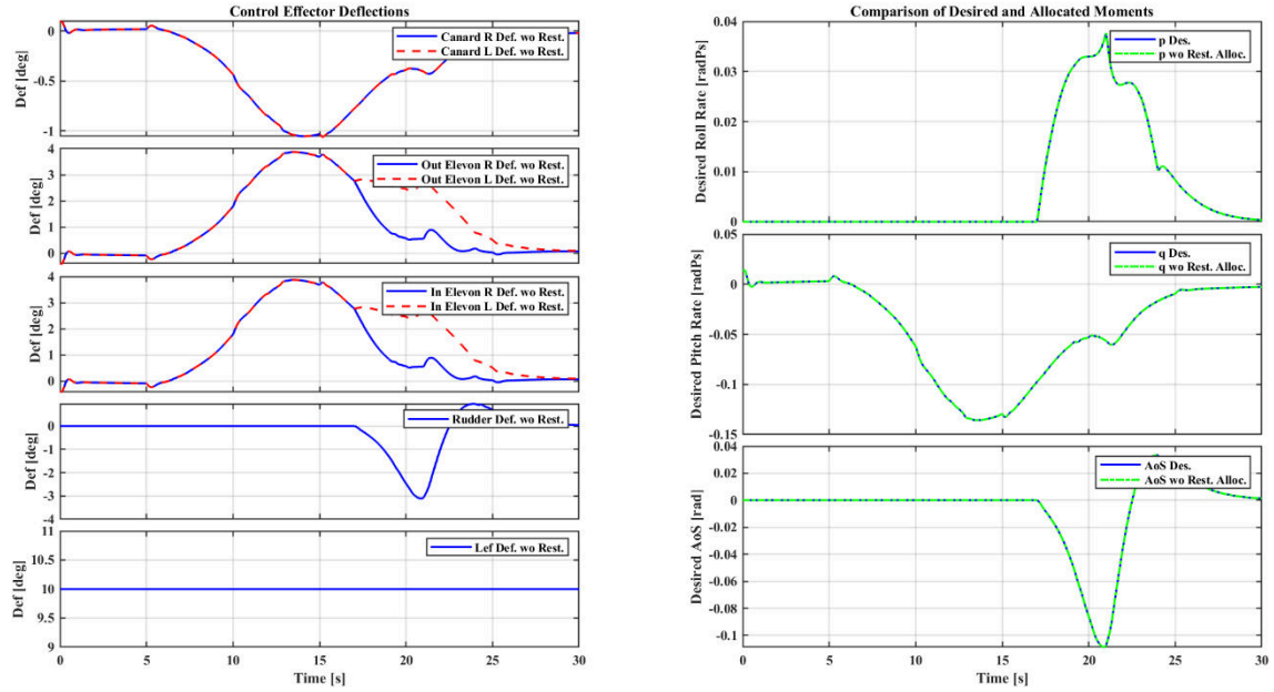
Figure 42: Scenario 2: Closed-Loop Results for Cascaded Generalized-Inverse Approach.
