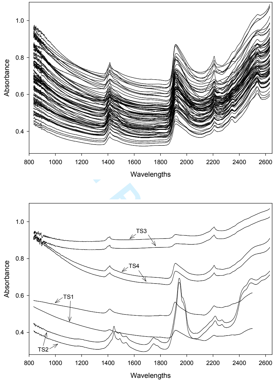
Supplementary content: Appendix I. Representative NIR spectra of the national samples included in the initial calibrations (top), and two representative NIR spectra of each of the four target sites (bottom).
