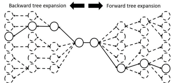
Figure 6. Backward and forward tree expansion for a given intermediate couple of asteroids. Bold nodes and branches belong to optimal sequence.
