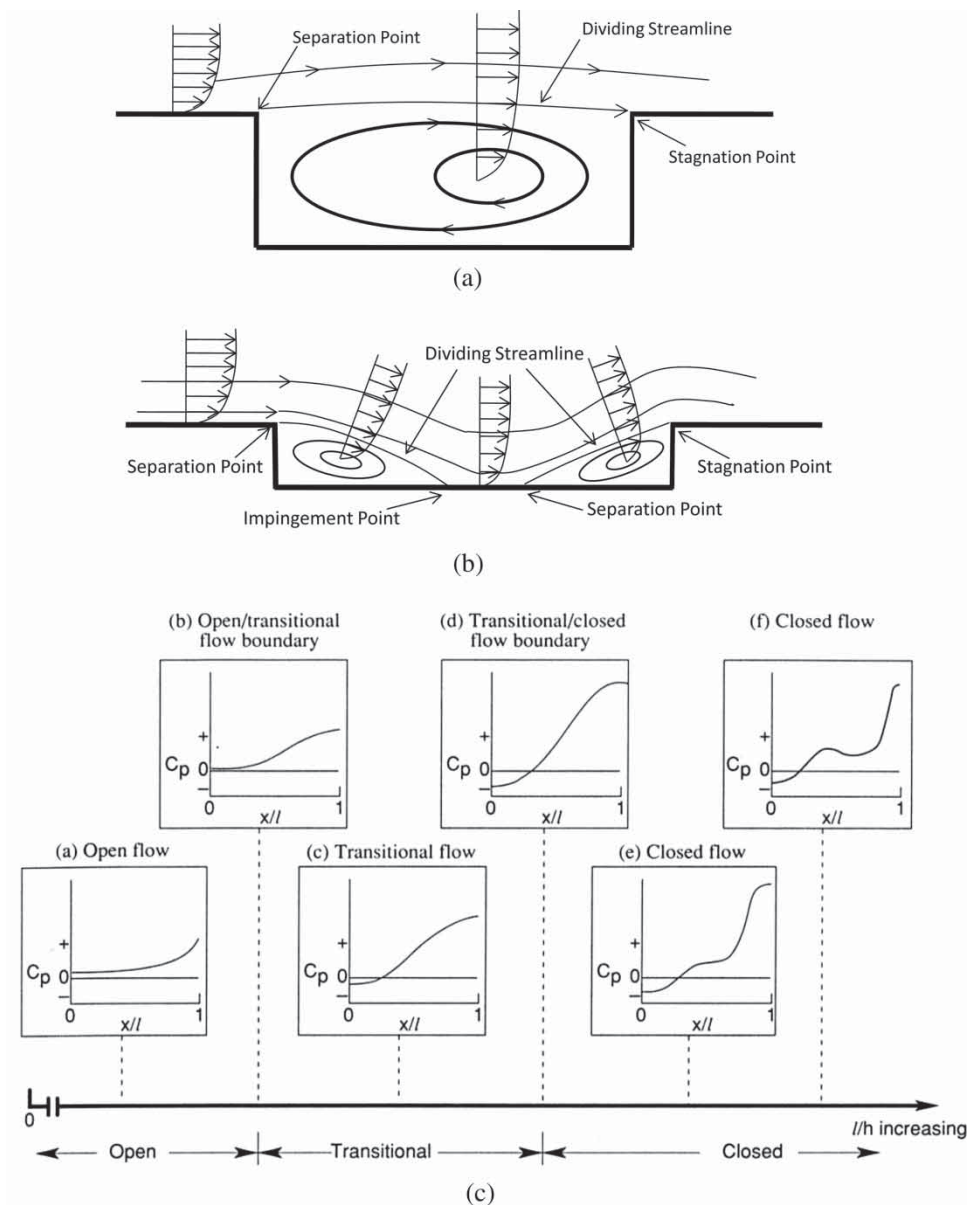
Fig. 1 Cavity flow types: (a) schematic of subsonic, open cavity flow; (b) schematic of subsonic, closed cavity flow; and (c) classification for subsonic flows, based on streamwise pressure gradient, after Stallings et al. [2]
