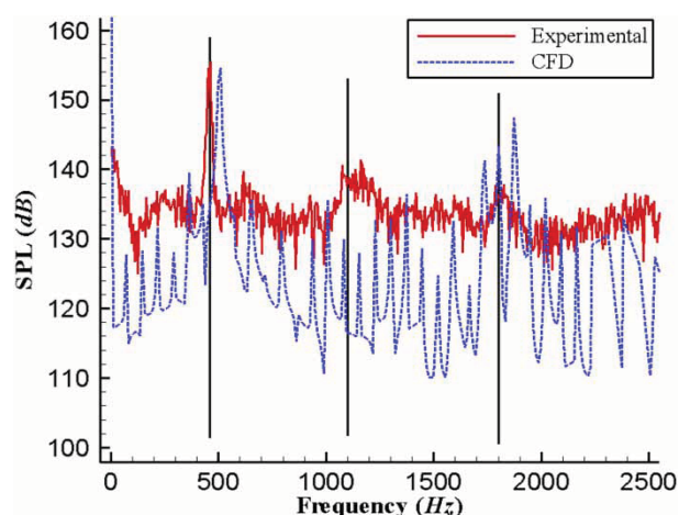
Fig. 6 Comparison of unsteady pressure spectra on centreline at x/L = 0.9 : experiment versus 3D CFD, half-domain simulation. Experimental spectrum has been adjusted for frequency response of apparatus. The vertical lines indicate the first three Rossiter modes according to equation (2)
