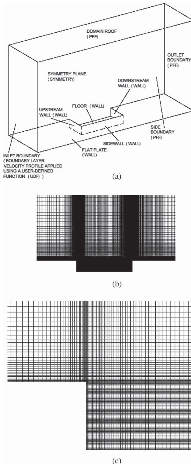
Fig. 4 CFD domain and grid: (a) domain construction and boundary type; (b) overview of grid in and around cavity; and (c) detail of grid around upstream cavity lip
