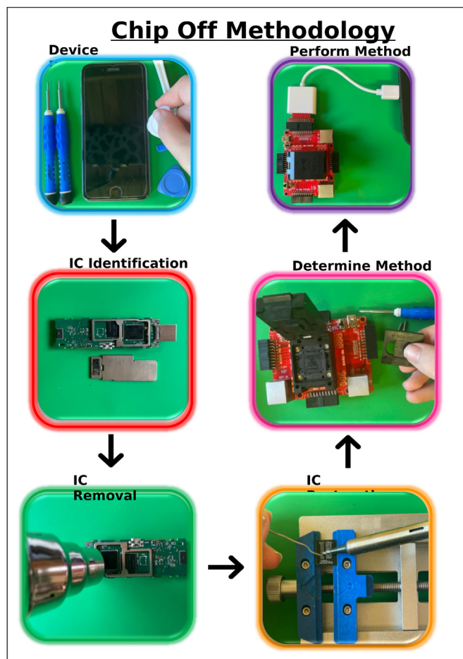
Fig. 6. Chip off methodology implementation images.
