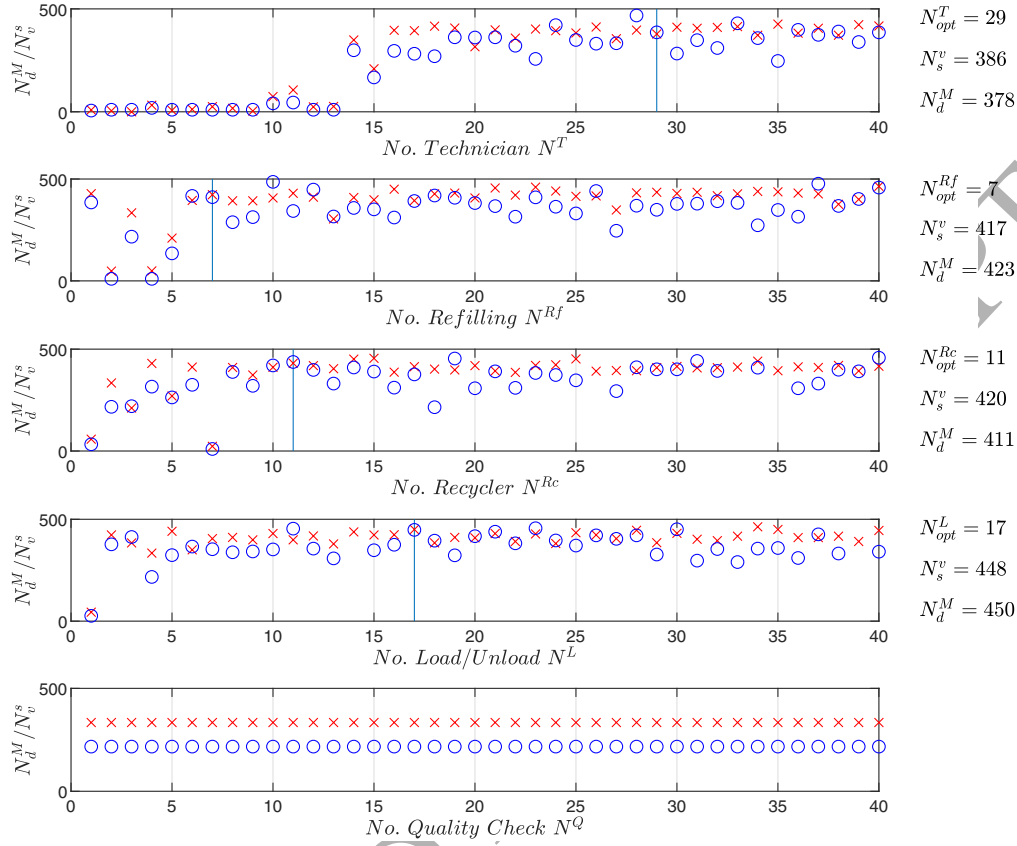
Figure 10: Parameters Variation experiment: number of staff members versus the monthly number of dispatches N_d^M with ( \times ) symbol, and validated shippers N_v^s with ( \circ ) symbol.
