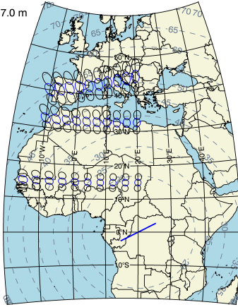
Fig. 1. Example C-band spot beam coverage, steerable over Europe and Africa by slewing the whole satellite (blue diagonal line is a representative relative orbit projected onto Earth; the dashed contours show local incidence angle).
