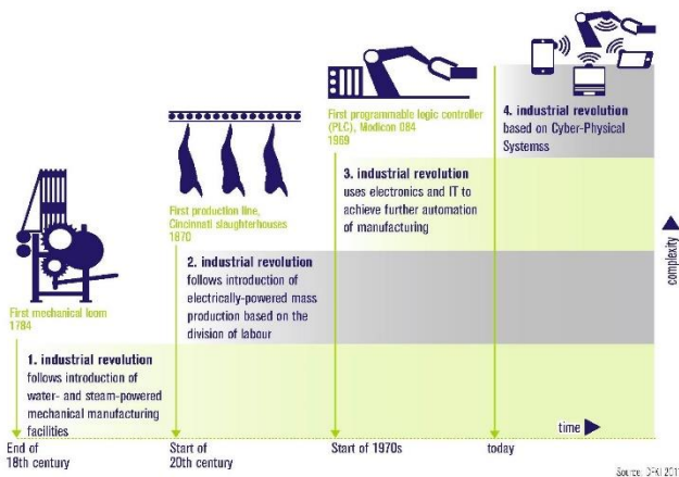
Fig.1. Industry 4.0 [4].
