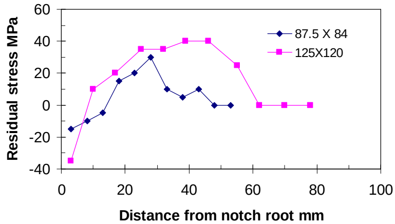
(b) Residual stress perpendicular to weld direction Fig. 8 Residual stress changes along the weld line across the sample width, for the two smallest CT samples (2 nd scan line)
