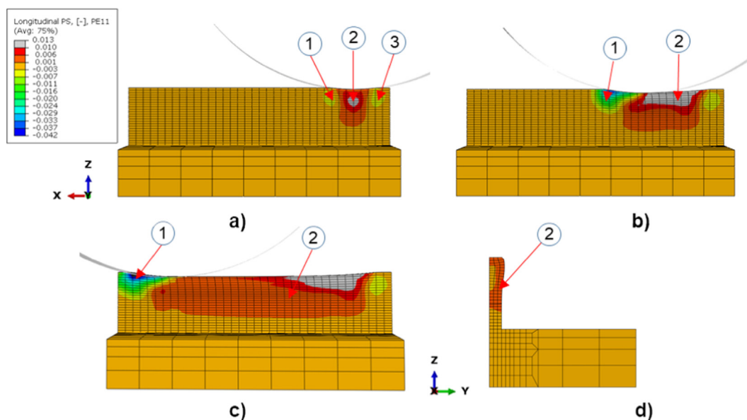
Fig. 6. Longitudinal PS generation during rolling with the flat roller ( F = 50 kN and \mu = 0.5 ): a) at the end of the establishment of contact in the loading step, b) at the beginning of the roller motion, c) at the end of the rolling step, and d) in the final rolling state on the transverse inspection plane. Note that in this analysis case the wall is assumed to be free from any strain and stress before rolling.
