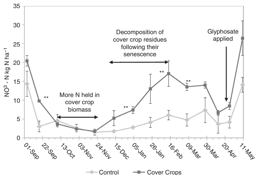
FIGURE 4 Topsoil \text{NO}_3\text{-N} ( \text{kg N ha}^{-1} ) measured between September 2017 and May 2018. Statistical significance is denoted by **, t -test ( p < .05 ). n = 3 , error bars = SEM
