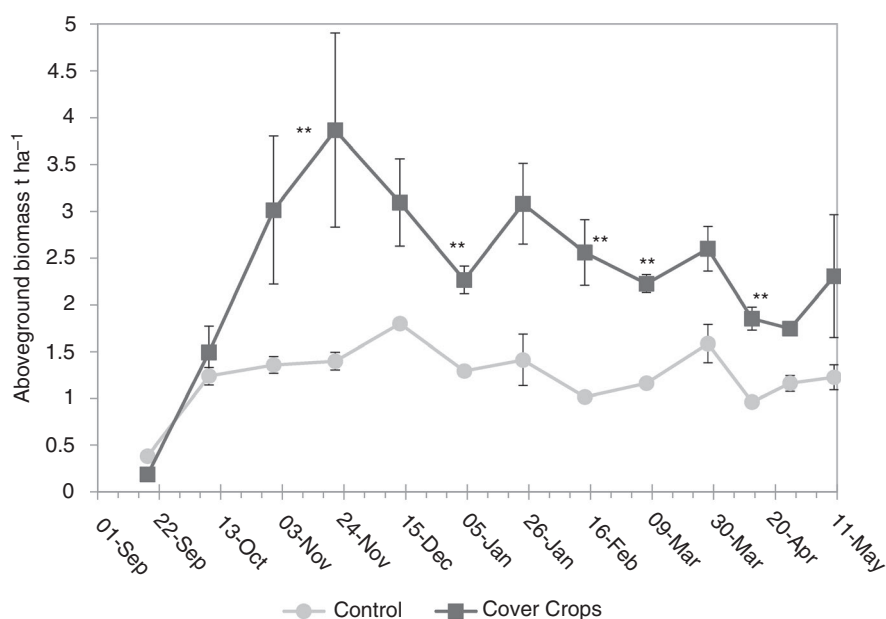
FIGURE 3 Dried above ground biomass measured between September 2017 and May 2018. Statistical significance is denoted by **, t -test ( p < .05 ). n = 3 , error bars = standard error of the mean (SEM)
