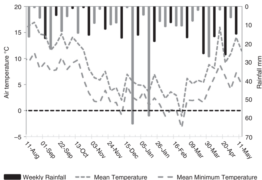
FIGURE 1 Weekly rainfall (mm), mean and minimum temperature ( ^\circ\text{C} ) recorded over the duration of the trial (2017 to 2018). Weekly rainfall (coloured in black) signified when a topsoil N and aboveground biomass sample was taken
