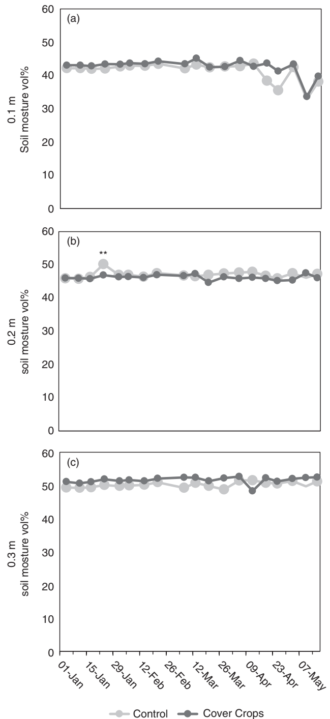
FIGURE 2 Mean soil moisture (Vol %) at 0.1, 0.2 and 0.3 m depths (a, b and c, respectively) in 2018. Statistical significance is denoted by **, t -test; p < .05 . n = 3 , unless data points were removed by the data screening process
