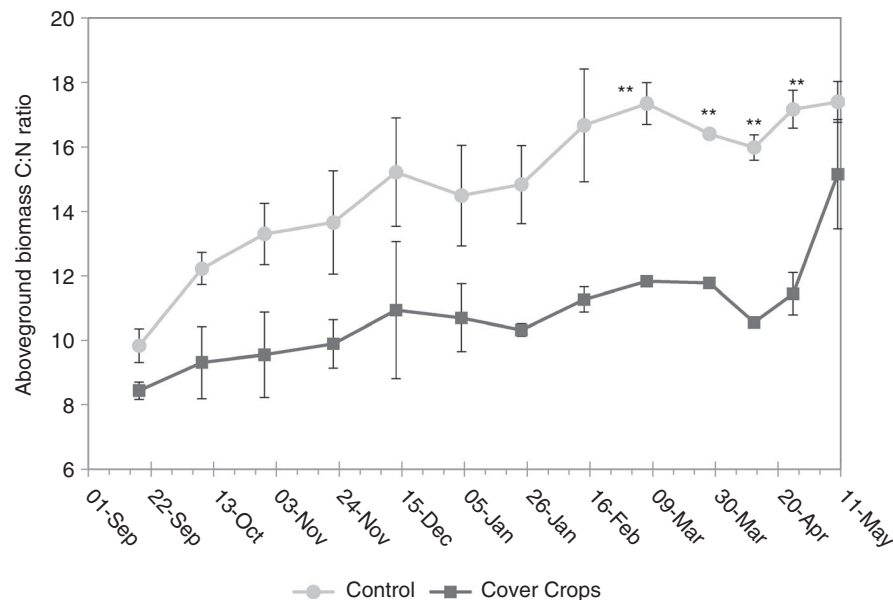
FIGURE 6 Above ground biomass C:N ratio between September 2017 and May 2018. Statistical significance is denoted by **, t -test ( p < .05 ). n = 3 , error bars = SEM
