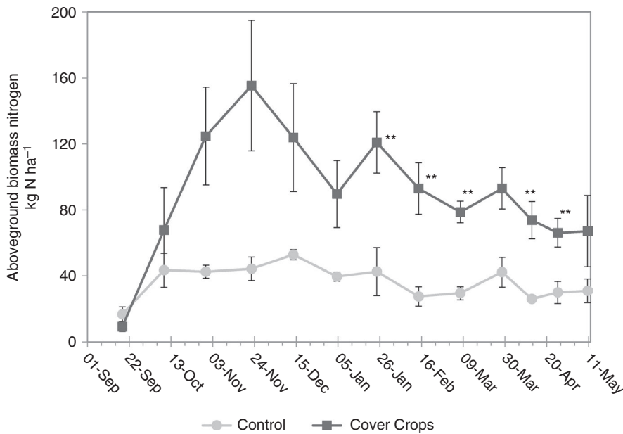
FIGURE 5 Above ground biomass N ( \text{kg ha}^{-1} ) measured between September 2017 and May 2018. Statistical significance is denoted by **, t -test ( p < .05 ). n = 3 , error bars = SEM
