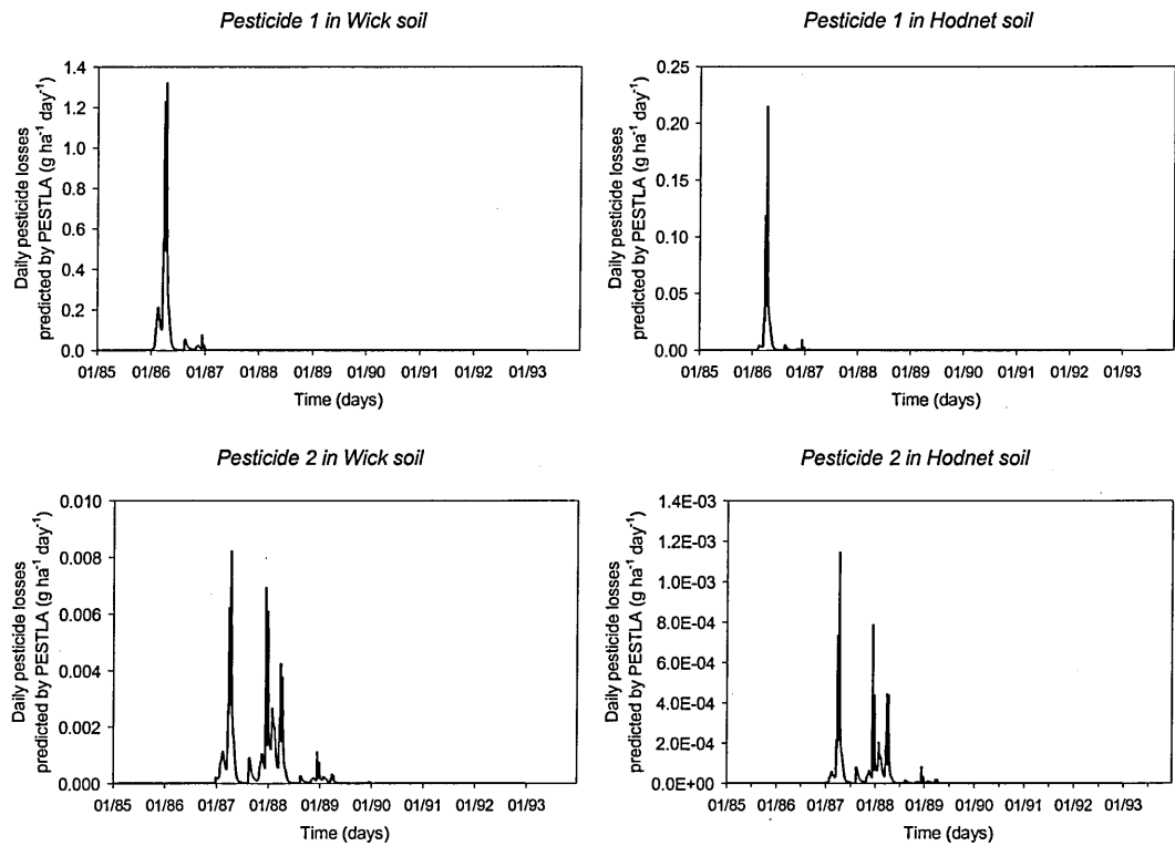
Figure 3-4. Daily predictions for pesticide losses by PESTLA for the four base-case scenarios.
