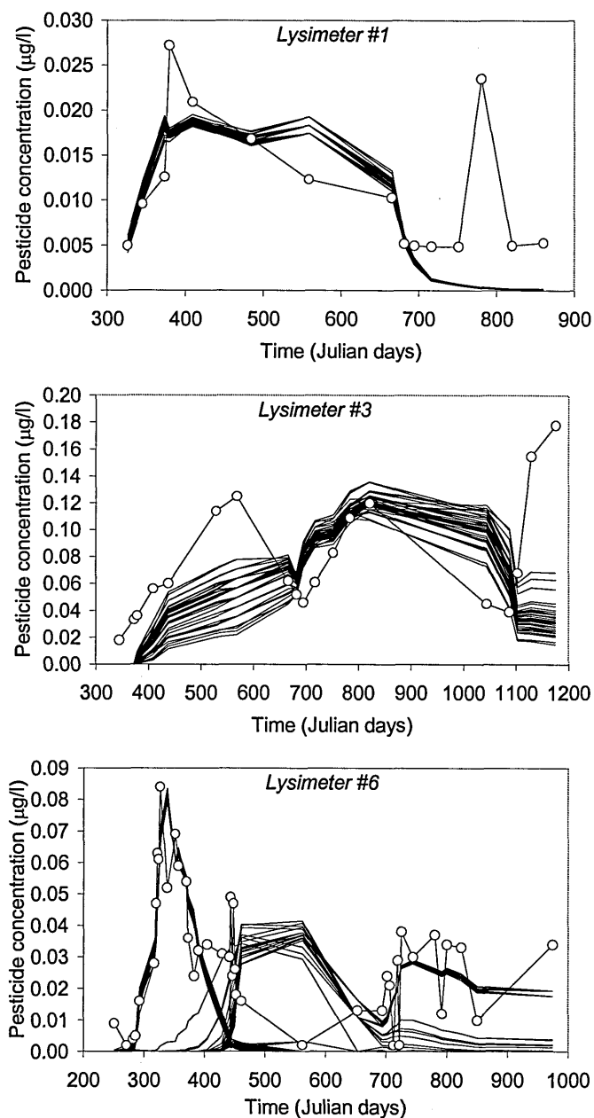
Figure 6-4. Pesticide breakthrough simulated after calibration of PESTRAS for different n_f values (plain lines). The experimental data are shown by open circles.
