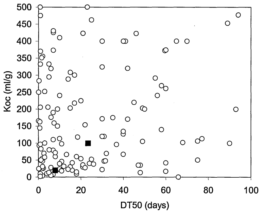
Figure 4-1. Comparison between K_{oc} and DT_{50} values of the two theoretical pesticides considered in the present study (closed squares) and those for pesticides registered for use in the UK (open circles). Properties for registered compounds were taken from Lewis and Bardon (1998). Only those registered pesticides with K_{oc} < 500 ml/g and DT_{50} < 100 days are shown.
