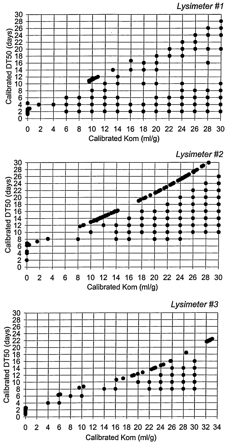
Figure 6-5. Combinations of calibrated K_{om} and DT50 values obtained for different starting values. Calibrated values are represented by closed circles. Starting values are represented by grid nodes.
