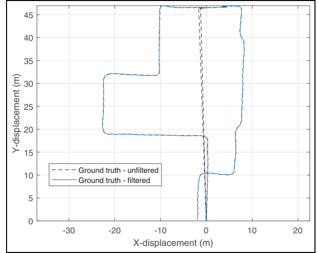
Figure 2. Hampel filter outlier replacement on ground truth trajectory data.
