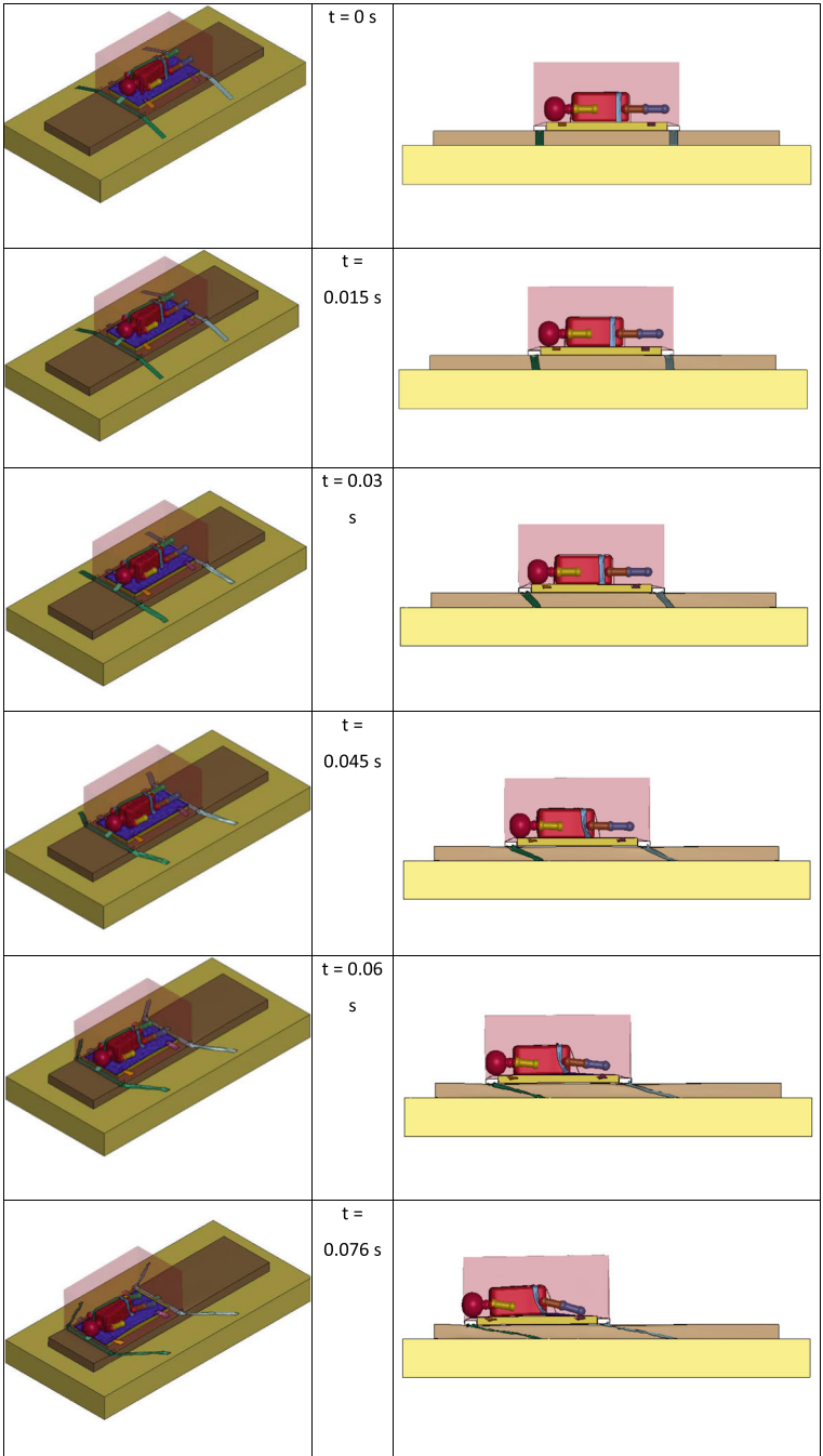
Fig. 8 Various stages of kinematics subjected to 10 g
