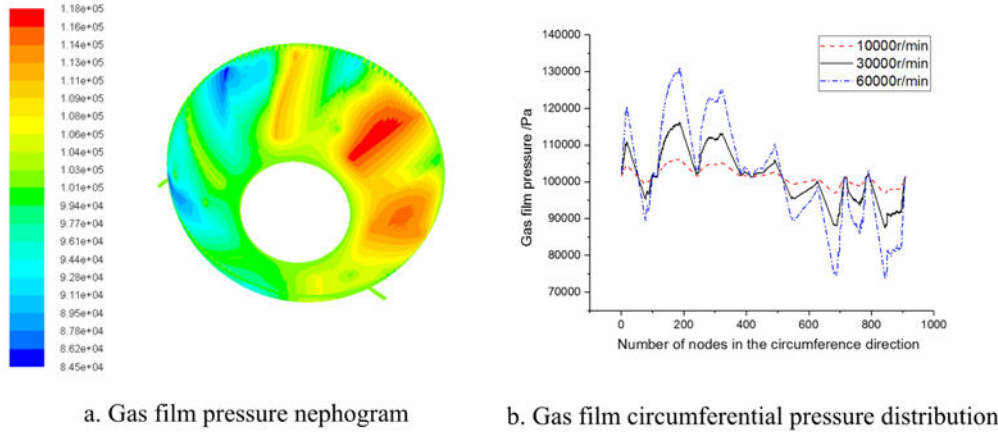
Fig. 7 Gas film pressure nephogram and circumferential pressure distribution at gas supply pressure of 0.11MPa
