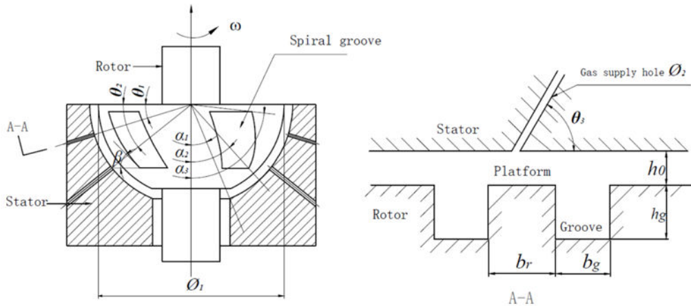
Fig. 1 Spherical spiral groove hybrid gas bearings profile diagram
