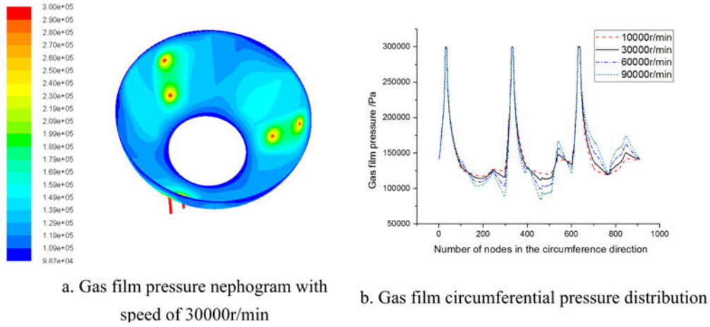
Fig. 8 Gas film pressure nephogram and circumferential pressure distribution at gas supply pressure of 0.3MPa
