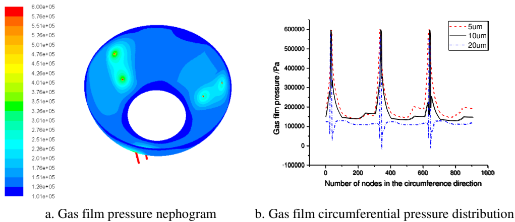
Fig. 6 Gas film pressure nephogram and circumferential pressure distribution of different gas film thicknesses
