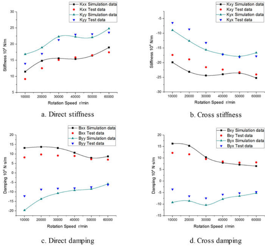
Fig. 19 Variation of rotation speed on dynamic stiffness and damping coefficients
