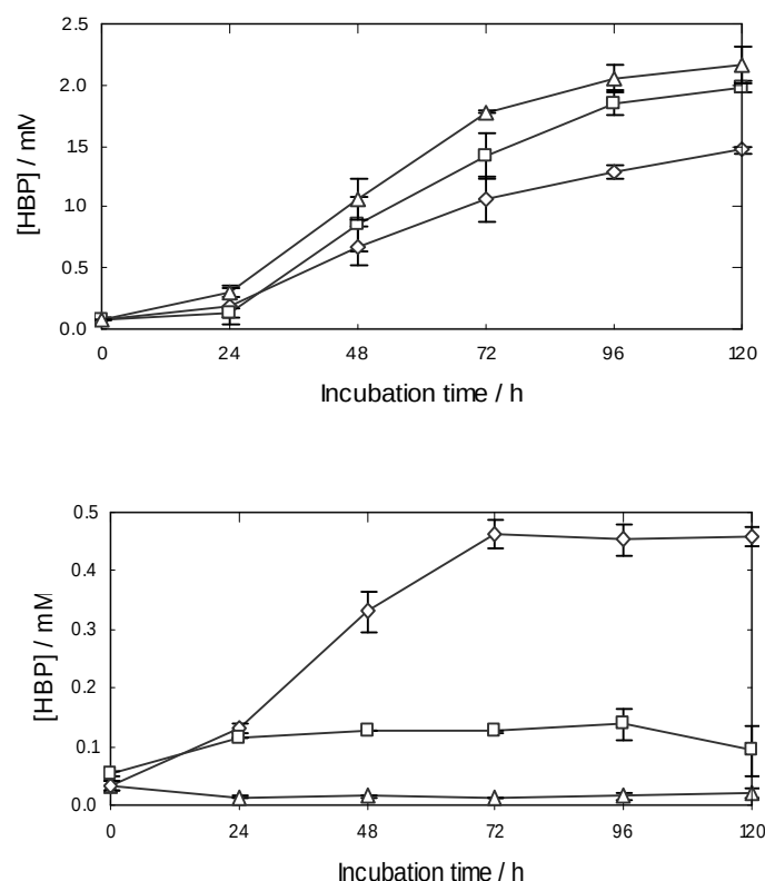
Figure 2. Production of HBP by (A) R. erythropolis and (B) S. putrefaciens at different concentrations of DBT. Key: ◇, 0.3 mM; □, 0.6 mM; △, 0.9 mM.
