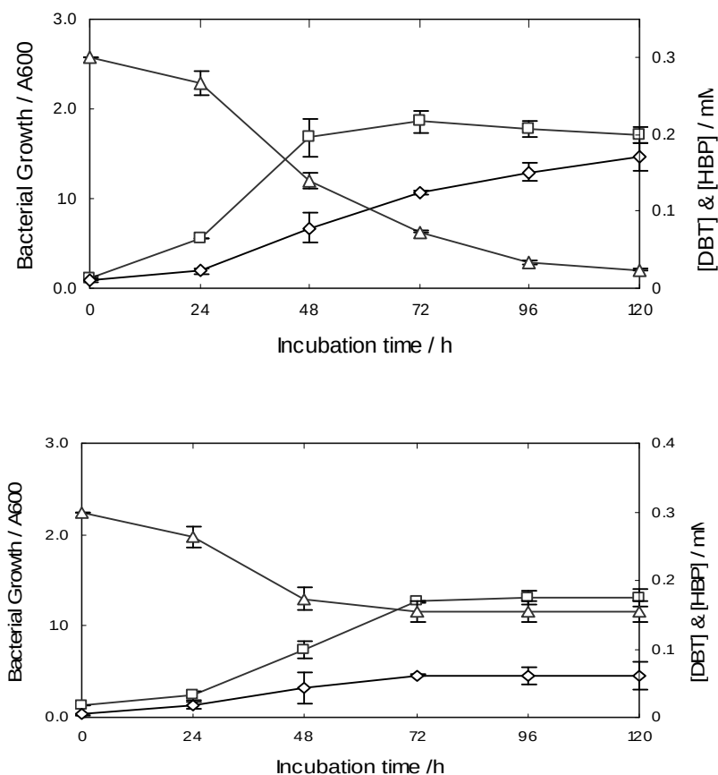
Figure 1. DBT desulfurization by (A) R. erythropolis IGTS8, and (B) S. putrefaciens NCIMB in DBT at a concentration of 0.3 mM as the sole sulfur source. Key: \square , bacterial growth; \square , concentration of HBP; \square , concentration of DBT.
