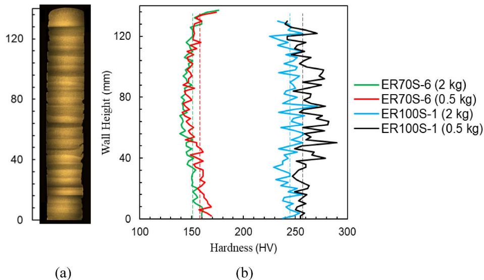
Fig. 4. (a) Macro structure of WAAM wall (b) Hardness test results for WAAM build walls.
