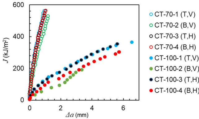
Fig. 7. Resistance curves for ER70S-6 and ER100S-1 specimens.
