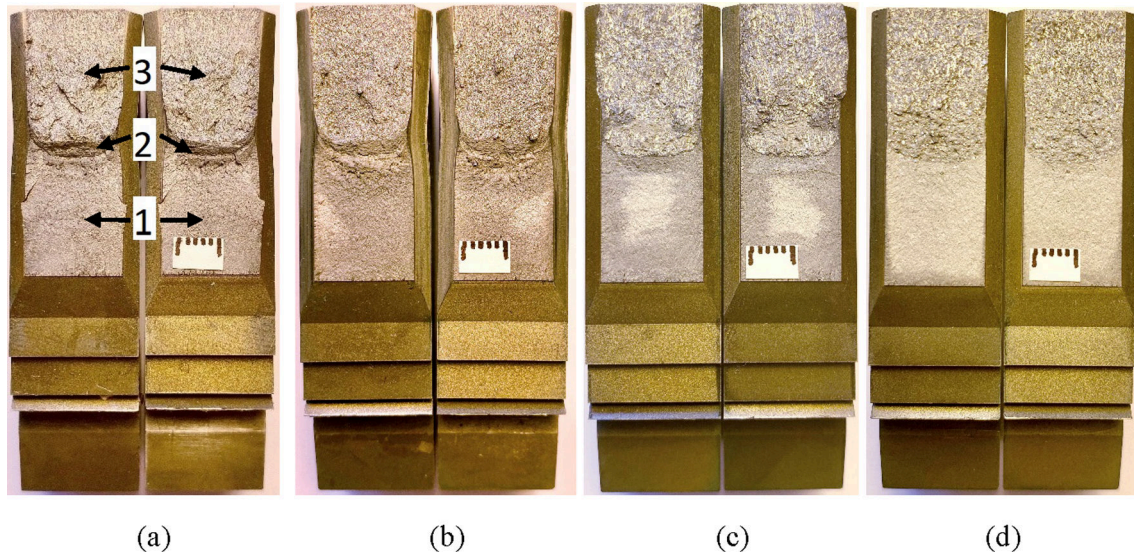
Fig. 9. Fracture surface for ER70S-6 specimen: (a) vertical CT-70-1, (b) horizontal CT-70-3; ER100S-1: (c) vertical CT-100-1, (d) horizontal CT-100-3.
