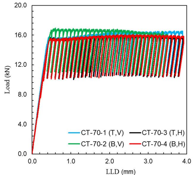
Fig. 5. Load vs. LLD for ER70S-6 specimens.
