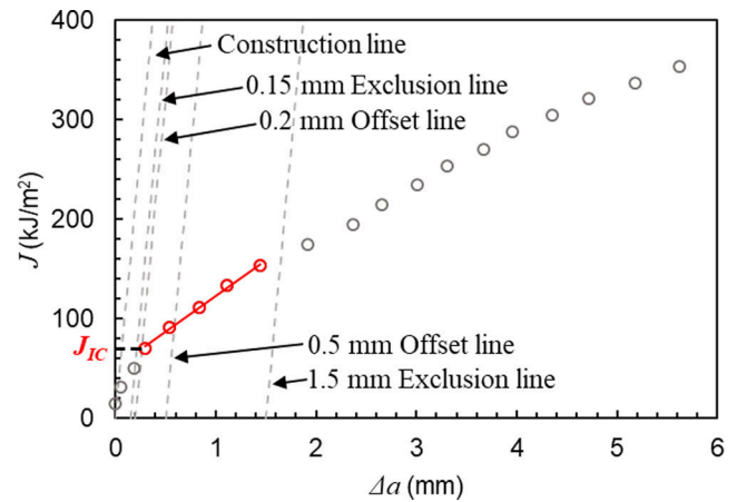
Fig. 8. Analysis of the fracture toughness data for CT-100-3 specimen.
