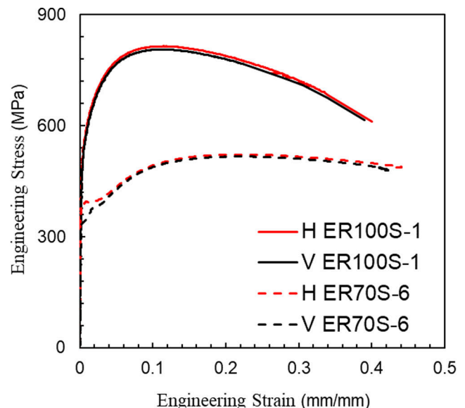
Fig. 3. Engineering stress-strain curves for the two studied materials.
