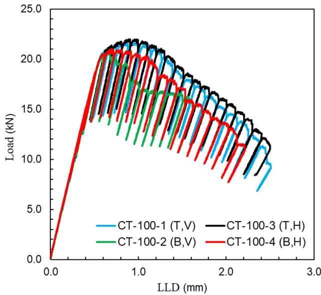
Fig. 6. Load vs. LLD for ER100S-1 specimens.
