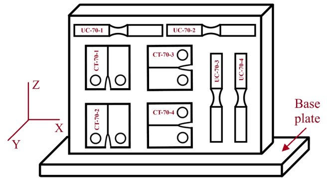
Fig. 2. A schematic demonstration of the specimen extraction plan.
