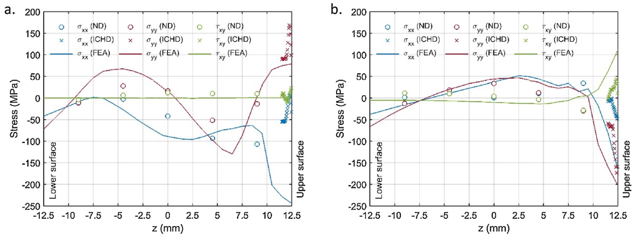
Fig. 11. Through-thickness comparison of residual stress data from Neutron Diffraction (ND), Incremental Centre Hole drilling (ICHD), and Finite Element Analysis (FEA) beneath the ICHD measurement locations shown in Fig. 1c a.) ICHD 1, b.) ICHD 2.
