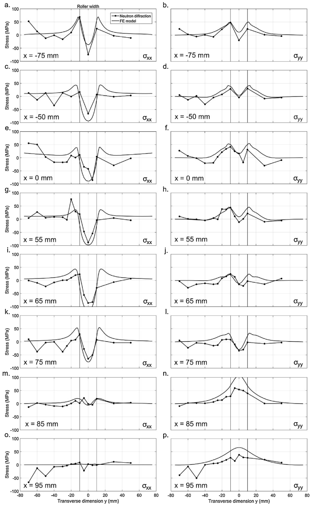
Fig. 10. Line plots longitudinal ( \sigma_{xx} ) and transverse ( \sigma_{yy} ) stress at the mid-thickness of the specimen ( z = 0 mm) at eight distances along the rolled region (see in Fig. 1c). The uncertainty in the experimental measurement is approximately \pm 20 MPa.
