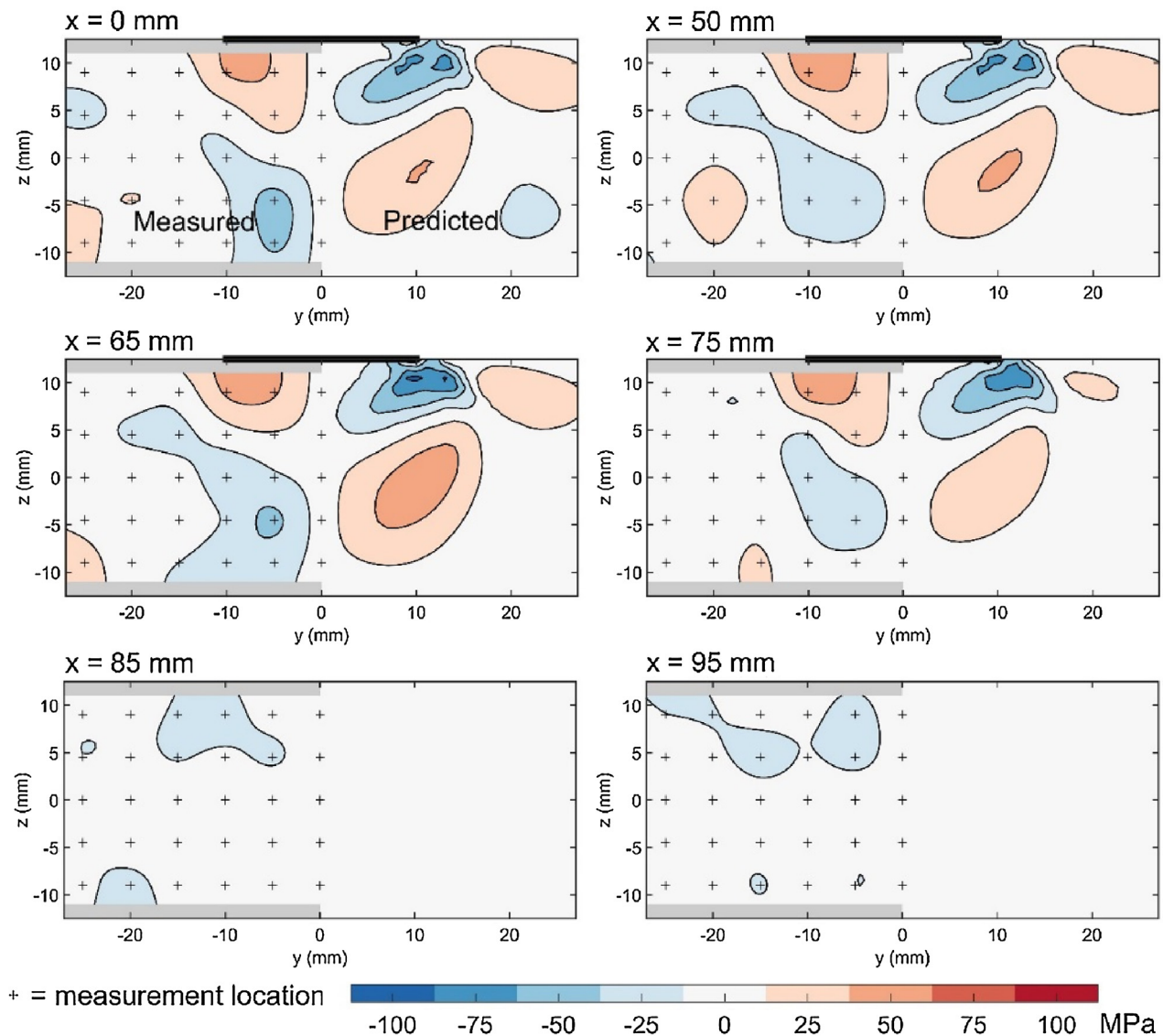
Fig. 9. Residual y-z shear stress ( \tau_{yz} ) on six y-z planes within the specimen. \tau_{yz} is anti-symmetric about the x-y plane. Black crosses indicate neutron diffraction gauge volume centres and black lines at z = 12.5 indicate the roller contact zone. Note different colour scale to Figs. 7 and 8.
