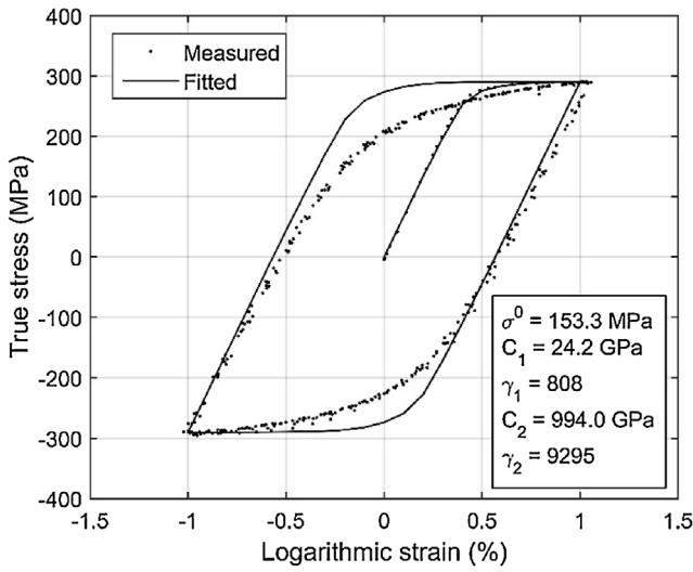
Fig. 3. Cyclic uniaxial stress-strain response of aluminium alloy 6082-T6 for a strain range of \pm 1\% . The response of a fitted Chaboche non-linear kinematic hardening model is also shown.
