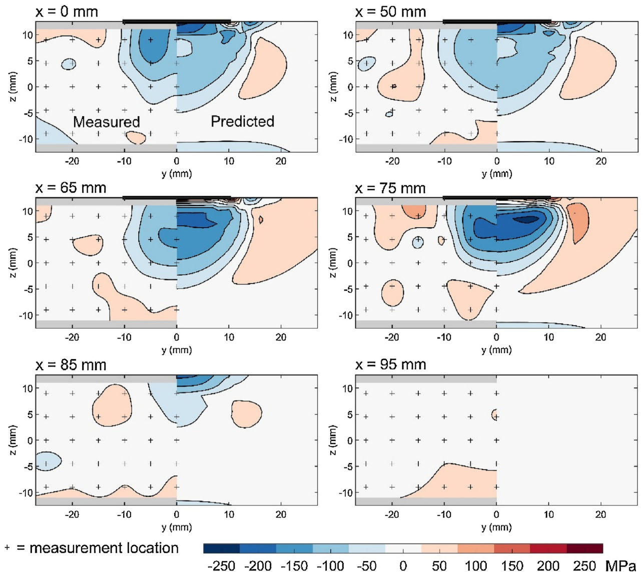
Fig. 7. Longitudinal residual stress ( \sigma_{xx} ) on six y-z planes within the specimen. Black crosses indicate neutron diffraction gauge volume centres and black lines at z = 12.5 indicate the roller contact zone.
