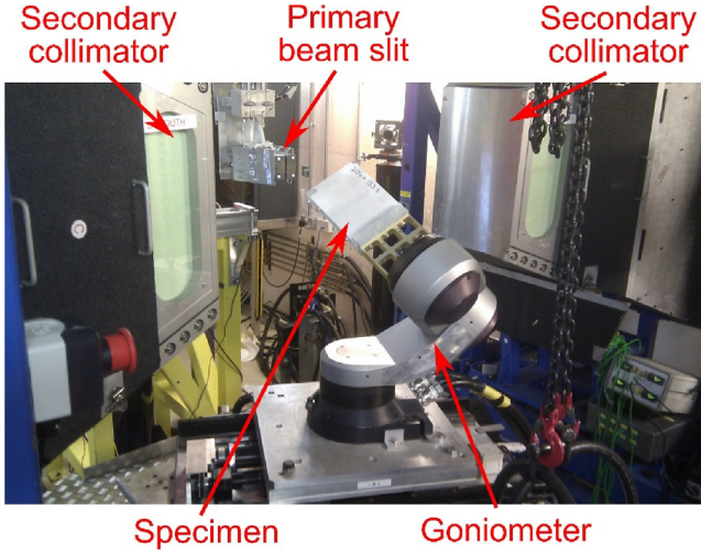
Fig. 4. Rolled plate specimen (painted white to allow specimen alignment using 3D laser scanning) set up and ready for measurement using the ENGİN-X neutron diffractometer. The goniometer was used to manipulate the specimen to achieve the scattering vectors shown in Fig. 5.
