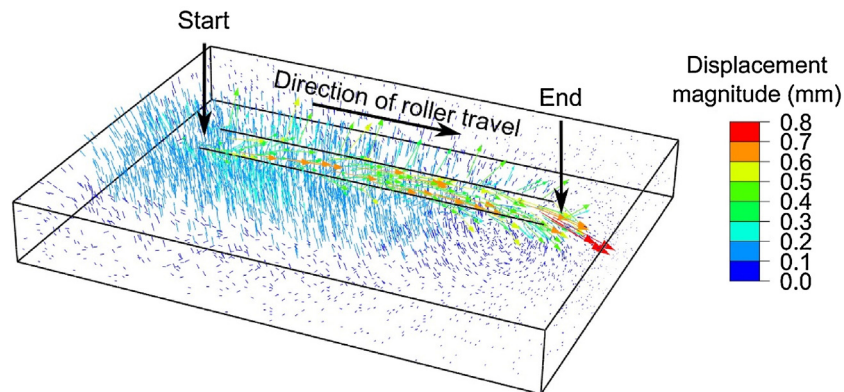
Fig. 13. Vector map of material displacement caused by rolling, as calculated using the FE model. Material directly under the roller is pushed down and forward. Meanwhile there is some uplift of material on the sides of the rolled region.
