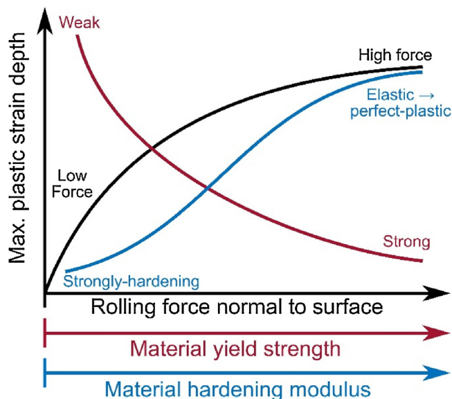
Fig. 15. Depth of effect of rolling as a function of material parameters and rolling force (schematic).
