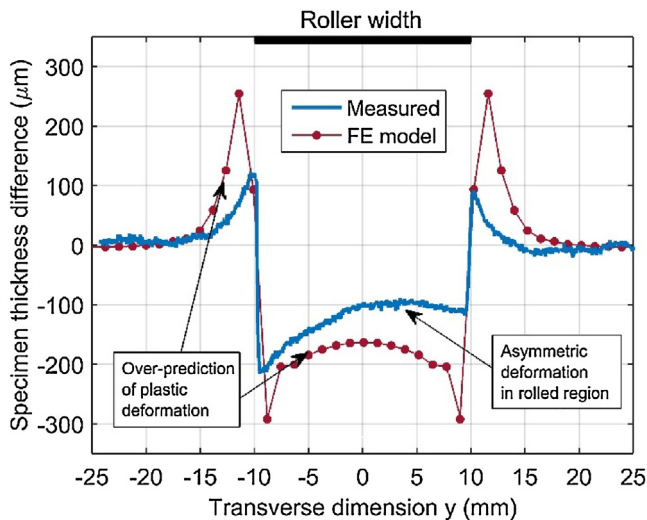
Fig. 14. The difference in specimen thickness produced by rolling, as predicted using FEA and measured using a contact profilometer.
