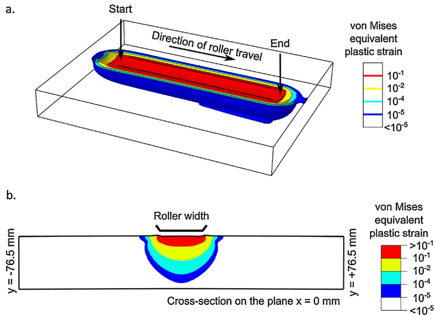
Fig. 12. Plastic strain distribution in the rolled plate after rolling predicted by finite element modelling of the rolling process. a.) Surfaces of constant plastic strain, b.) cross-section half-way along the length of the specimen ( x = 0 mm). Note the logarithmic scale.
