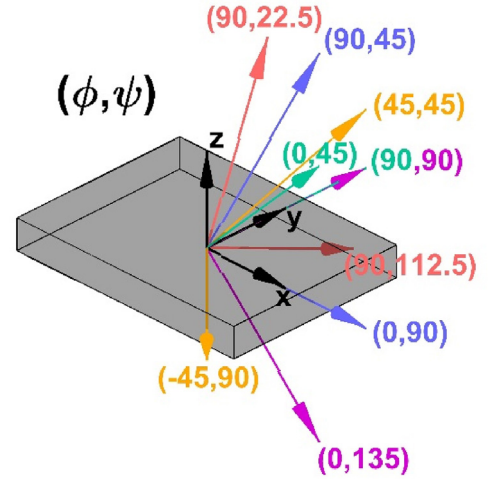
Fig. 5. Directions in which residual elastic strain was measured using neutron diffraction at the points shown in Fig. 1c. Angles in degrees. Pairs of arrows with the same colour indicate measurements made simultaneously using the two detector banks of ENGİN-X. Two sets of measurements were taken in the direction (90,90).
