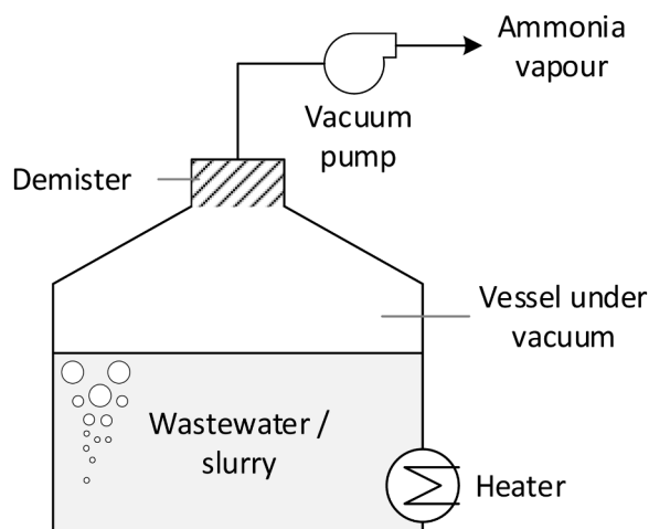
Fig. 6. Lab-scale setup for batch removal of ammonia from wastewater by vacuum thermal stripping.
