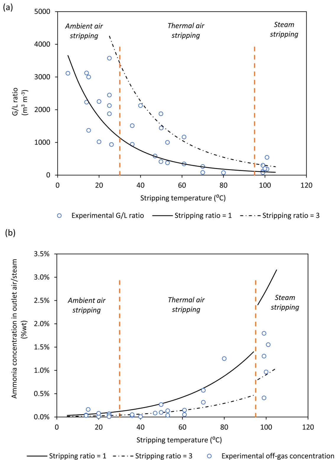
Fig. 5. Influence of temperature on (a) G/L ratio and (b) ammonia concentration in outlet gases for air and steam strippers (Quan et al., 2014; Değermenci et al., 2012; Bonmati and Flotats, 2003; Liu et al., 2015; Ferraz et al., 2013; Melgaço et al., 2020; Kim et al., 2021; Zeng et al., 2006; Serna-Maza et al., 2014; Quan et al., 2009; Katehis et al., 1998; Alitalo et al., 2012; Gopalakrishnan et al., 2000; EPA, 1992; Teichgraber and Stein, 1994; Boardman and McVeigh, 1998; Guštin and Marinšek-Logar, 2011; Jiang et al., 2010).
