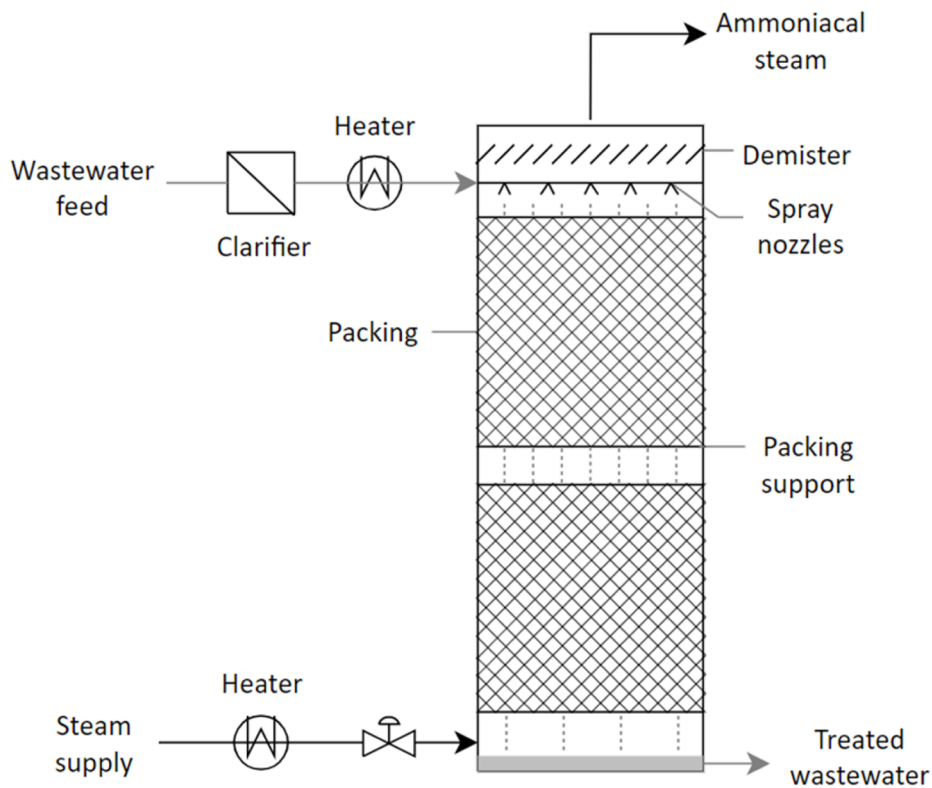
Fig. 2. Simplified flowsheets for continuous ammonia removal by (a) air stripping and (b) steam stripping in packed columns.
