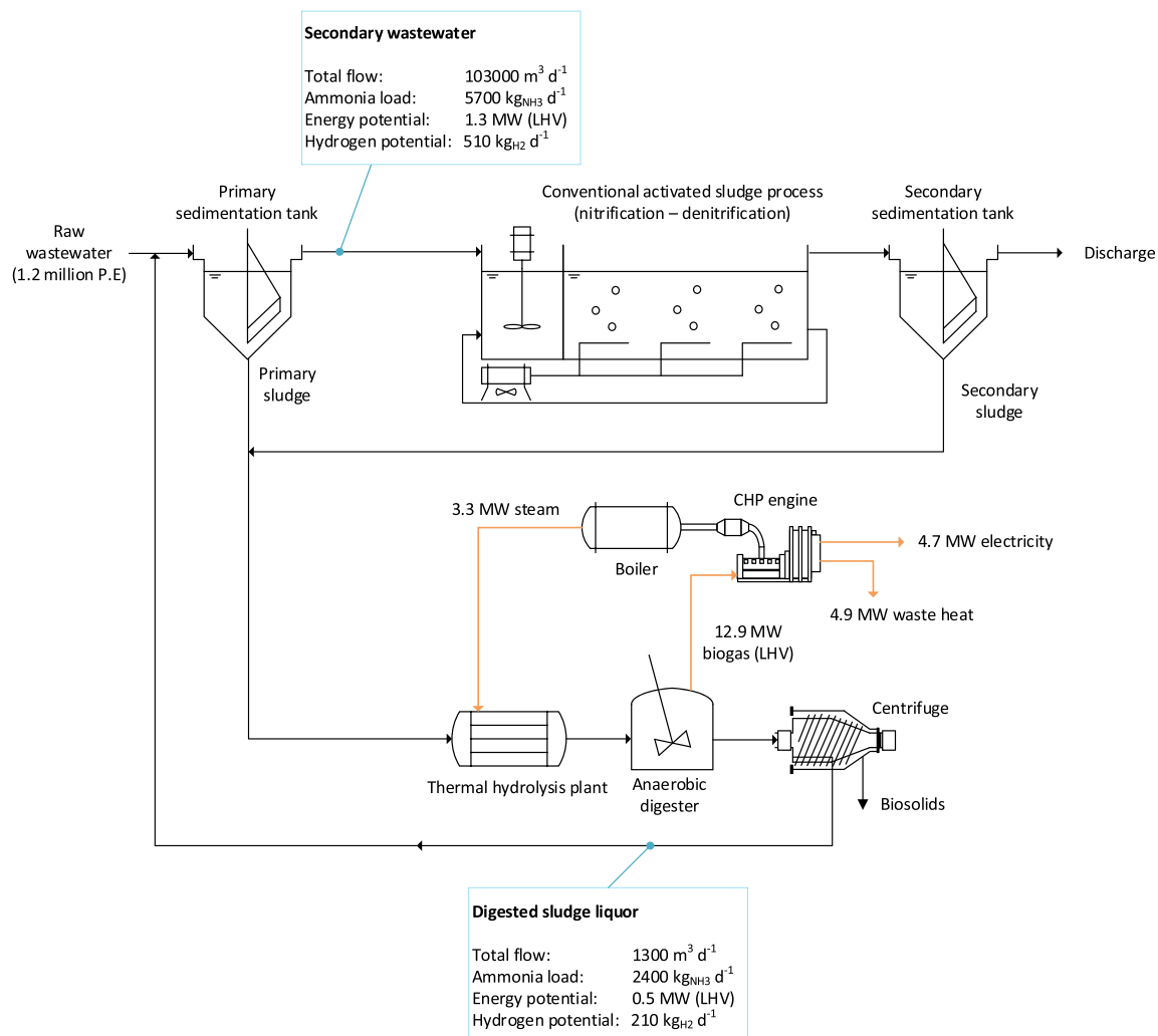
Fig. 1. Example wastewater treatment works with 1.2 million P.E. design capacity treating influent from domestic and industrial sources (Moore and Auty, 2013; Ndam, 2017).
