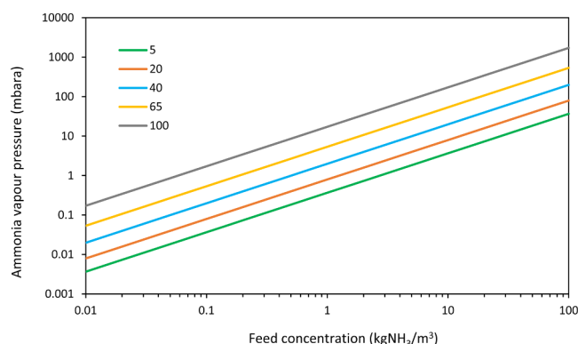
Fig. 4. Influence of temperature and concentration on ammonia vapour pressure exerted by feed. Derived from Henry’s law data for ammonia (National Institute of Standards and Technology, 2024).
