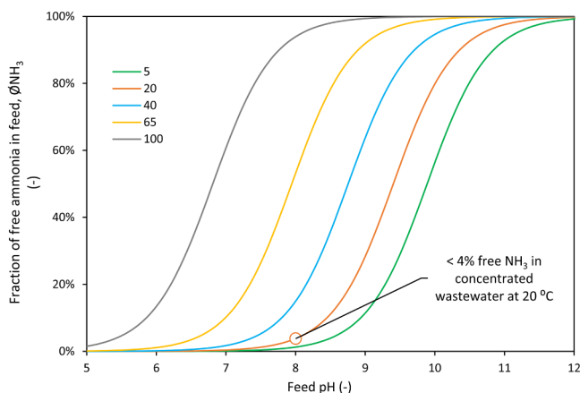
Fig. 3. Influence of temperature and pH on free ammonia fraction in feed. Derived from ammonia-ammonium equilibrium data (Bates and Pinching, 1949).
