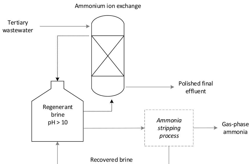
Fig. 8. Integrated ion-exchange-stripping process for ammonia recovery and wastewater polishing.
