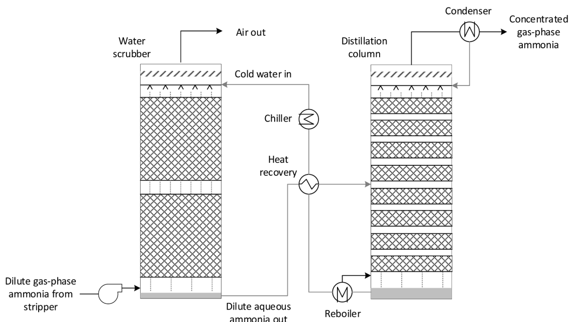
Fig. 7. Water scrubbing and distillation recovery flowsheet for dilute gas-phase ammonia concentration.
