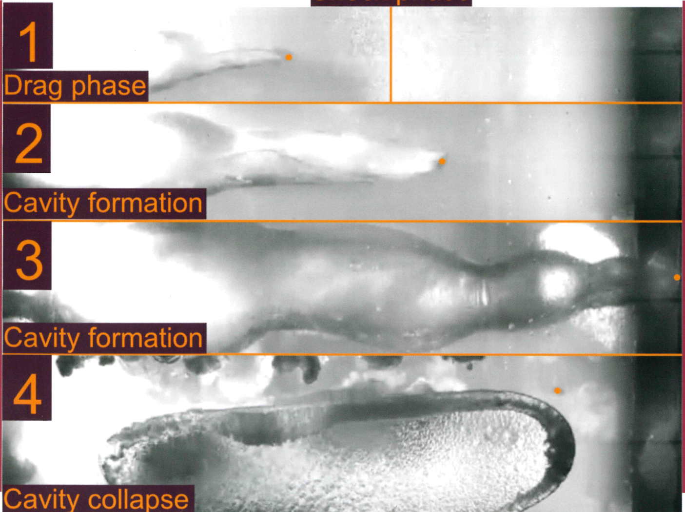
Figure 4: The cavitation and drag effects produced from a 7.62x39mm steel ball fired into the tank containing water at ~770m/s.
