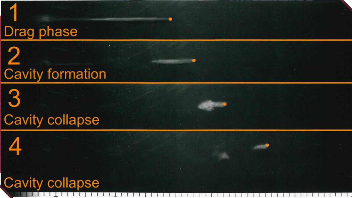
Figure 3: The cavitation and drag effects produced from an 8mm steel ball fired into the tank containing water at 250m/s.
