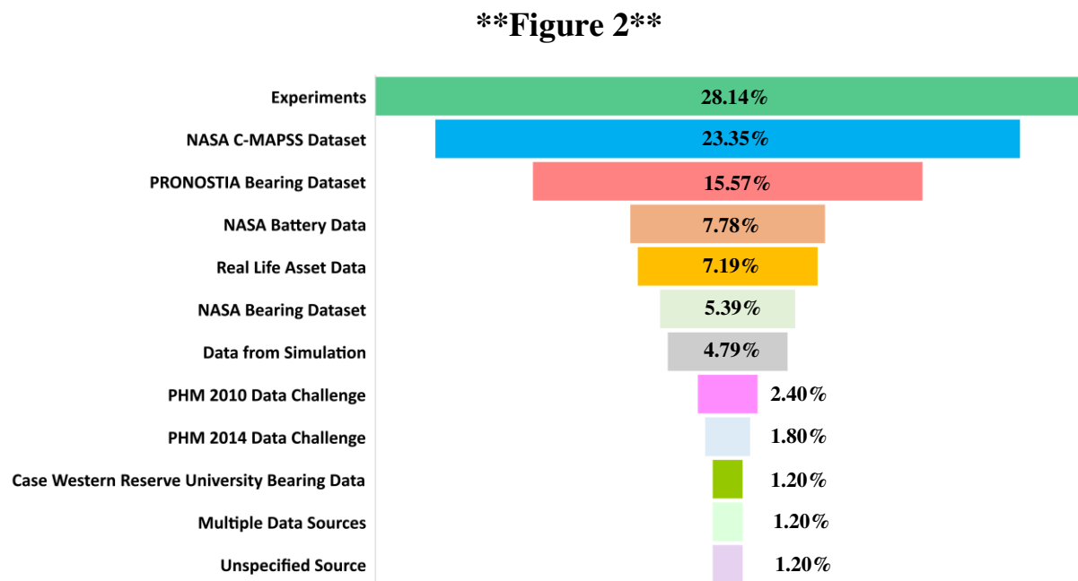
Fig. 2. Different datasets adopted in PHM research.
